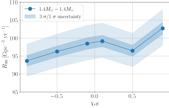
Figure 5. The 90% rate upper limit of 1.4 - 1.4 M_\odot compact binaries as a function of \chi_{\text{eff}} . The shaded regions denote the 3\sigma and 1\sigma Monte Carlo integral uncertainty.
