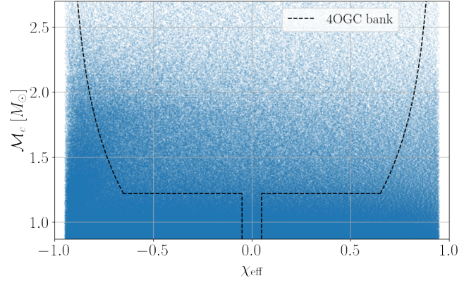
Figure 3. The template bank used in this search is plotted in the chirp mass and effective spin plane. Each point corresponds to a template, totaling \sim 700,000 . The dashed line denotes the boundary of the template bank used in 4-OGC as a comparison.
