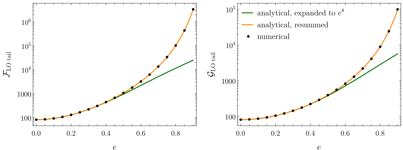
FIG. 1. The leading-order tail part of the energy (left panel) and angular-momentum (right panel) fluxes, plotted on a log scale. The resummed analytical expressions are much closer to the numerical results of Ref. [58] than the eccentricity-expanded expressions, even for eccentricities close to one.
