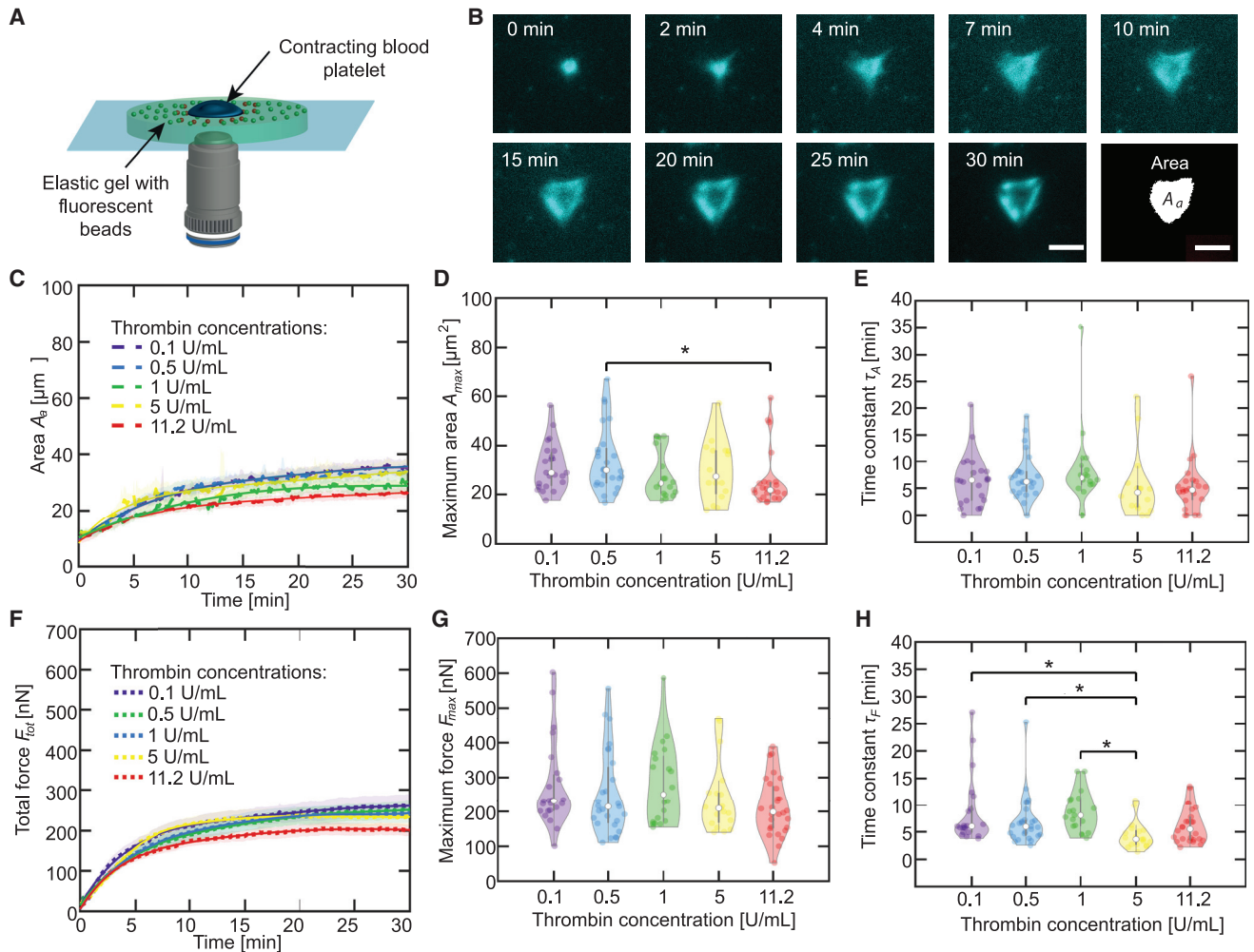
FIGURE 1 Above a threshold, thrombin concentration has no systematic effect on platelet spreading and force generation. (A) Schematic representation of the experimental setup. A contracting platelet (blue) on top an elastic gel (light green) displaces the fluorescent beads (green). The deformation of the gel due to the contraction is visualized as orange beads. (B) Epifluorescence micrographs of a blood platelet stained for actin and spreading on an elastic gel after stimulation by thrombin. The last image shows a binarized version of the t = 30 min micrograph. The scale bars correspond to 5 \mu\text{m} and refer to all sub-panels. The example platelet shown here is also shown in Figs. 3, 4 A , and 5 . (C) The average time-dependent total area covered by actin structures A_a(t) upon stimulation by different concentrations of thrombin. Each averaged curve contains a minimum of 18 datasets and the SEs are shown as the transparent areas. Averaged exponential fits are shown as solid lines. (D) Maximum areas for each dataset determined from the averaged total A_a(t) curves shown in (C). (E) Time constants for each dataset determined from the averaged total A_a(t) curves shown in (C). (F) Average total force curves for blood platelets ( n \geq 18 ) upon stimulation by different concentrations of thrombin are shown as dotted lines, and the SEs are included as the transparent areas. Averaged exponential fits are shown as solid lines. (G) Maximum forces for each dataset comprising the averaged total force curves shown in (F). (H) Time constants for each dataset comprising the averaged total force curves shown in (F). The violin plot outlines illustrate the kernel probability density; the width of the shaded area represents the proportion of the data points located there. In each violin plot, the white circle indicates the median, the thick gray bar indicates interquartile range, and the thin gray line indicates the full range of distribution without outliers. Experimental conditions with a statistical difference below a 5% significance level are marked by asterisks (*). To see this figure in color, go online.
