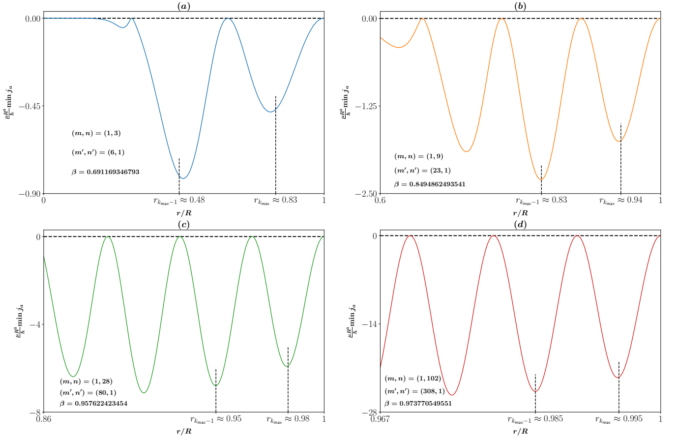
FIG. 1. (Dimensionless) minimum current (\mu R^3/\hbar) \min j_a , as given by (B9), as a function of the (dimensionless) radial coordinate r/R for the four sets of parameters (m, n, m', n', \beta) considered in Table I. The corresponding values of the positions r_{k_{max}-1} and r_{k_{max}} are also indicated.
