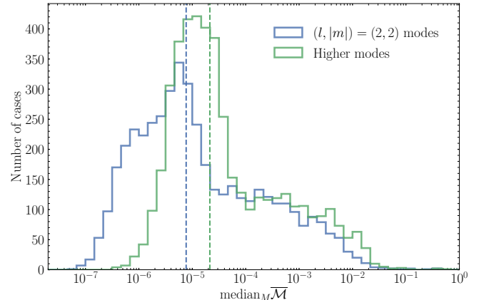
Figure 3. Distribution of median unfaithfulness over the total mass range between [20 - 300]M_\odot for an inclination \iota = \pi/3 , between the (l, |m|) = (2, 2) -modes models, SEOBNRv4E and SEOBNRv4E_opt (blue), as well as between the higher-order mode models, SEOBNRv4EHM and SEOBNRv4EHM_opt (green) for 4500 configurations in the parameter space q \in [1, 50] , \chi_{1,2} \in [-0.9, 0.9] , e_0 \in [0, 0.5] and \zeta_0 \in [0, 2\pi] for a dimensionless starting frequency of M\omega_0 = 0.023 . The vertical dashed lines indicate the median values of the distribution.
