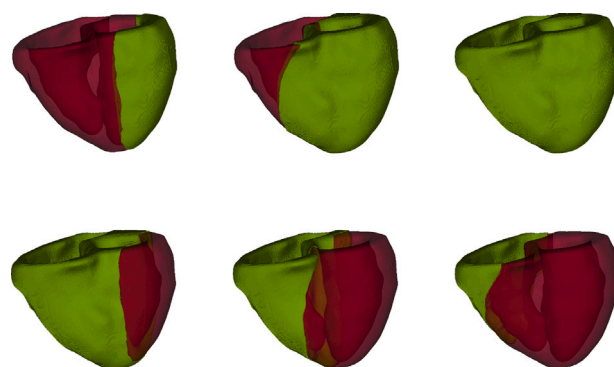
Fig. 17. Two-level isosurface plots of V for the 3D TP06 model illustrating a wave passing from one end to the other of our 3D realistic, human-heart geometry in the normal situation (without any obstacles). The upper panels show the initial stages from left to right; the lower panels show the wave finally moving out of the medium (cf. Fig. 9 for the 3D HRD model). For the complete spatiotemporal evolution see the Videos S22 in the Supplementary Material [29].
