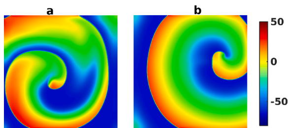
Fig. 5. Pseudocolor plots of the transmembrane potential V showing the two major types of spiral arms we observe in our 2D HRD-model simulations: (a) a spiral with a nonuniform wave width in different regions, with much thinner arms than in the center; and (b) a spiral with an almost uniform arm width. For the complete spatiotemporal evolution see the Videos S33 and S34 in the Supplementary Material [29].
