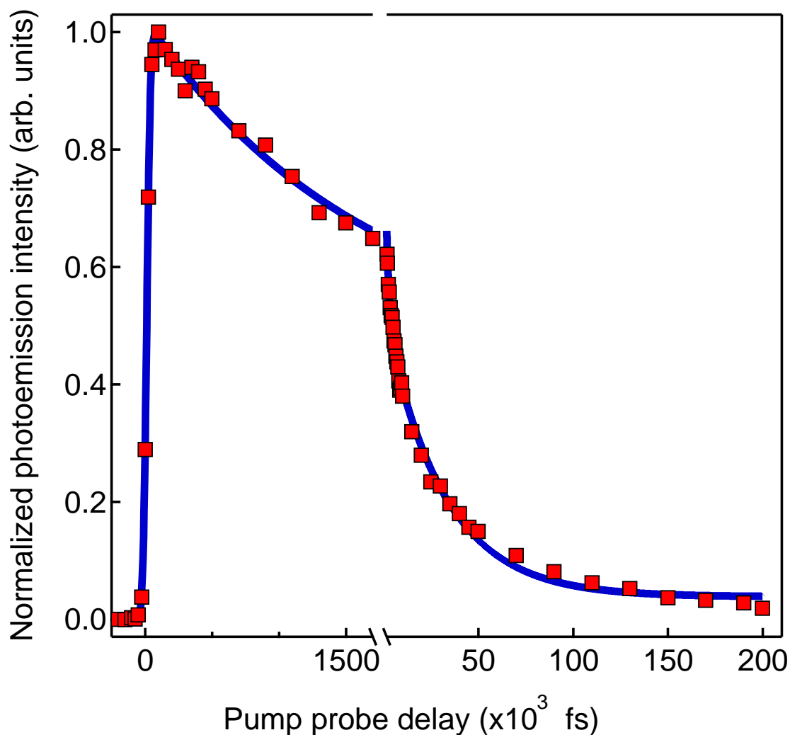
Figure S5: Long delay \Sigma valley population for pure WSe 2 . Combination of data and fit for pure WSe 2 measured with 800 nm pump, 0.6 mJ/cm 2 fluence. The long delay range shows a two timescales decay.
