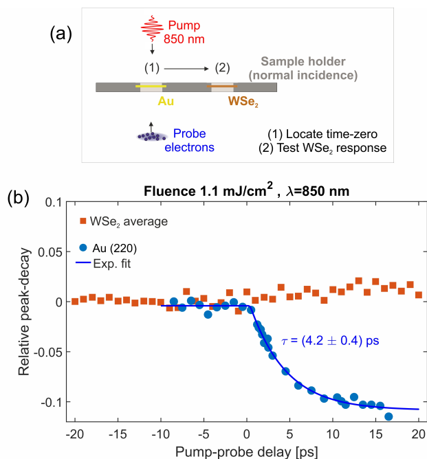
Figure S10: No lattice response of bare WSe 2 flakes exposed to sub-band-gap light. (a) The experiment used for finding temporal overlap of pump and probe and then testing the lattice dynamics of bare WSe 2 . (b) The relative peak-decay for the (220) peak of a Au thin-film and for the average of the WSe 2 peaks.
