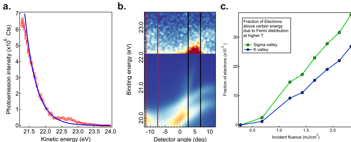
Figure S6: Analysis of 1030 nm measurements. a. Typical result of background fitting for the extraction of fluence dependence of \Sigma valley population. The fluence is 1.66 \text{ mJ/cm}^2 , the delay +400 \text{ fs} . The red circles show the data as obtained from tr-ARPES signal integration in the momentum range shown in panel b by the red lines. The blue curve shows the exponential background. b. tr-ARPES map with 1030 nm pumping. The red lines mark the range of integration for the EDC used for \Sigma valley population extraction, while the black lines show the range for Fermi edge fitting. c. Plot of the integral of the Fermi-Dirac distribution between the energy of the \Sigma and K valley and infinity, as a function of the electronic temperatures corresponding to the fluences used in Fig.3d.
