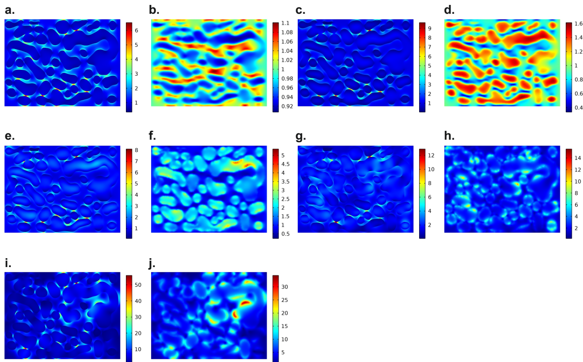
Figure S2: Electric field enhancement at various wavelengths. a.-b. Electric field enhancement in Au nanoislands on WSe 2 2 nm above (a.) and 1 nm below (b.) the interface, with 400 nm excitation. c.-d. Same, but for 800 nm excitation. e.-f. Same, but for 860 nm excitation. g.-h. Same but for 1060 nm excitation. i.-j. Same, but for 1200 nm excitation.
