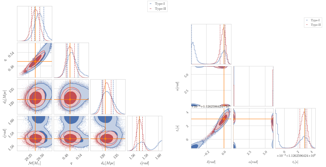
Figure 6. The recovery of source parameters using Type-I (blue) and Type-II (red) templates for q = 2 , M = 70M_{\odot} , \rho = 50 , and \iota = \pi/2 . The Type-II recoveries are consistent with the injection values, but the Type-I recoveries have correlated bimodalities t_c , \delta and \iota . One of these modes is consistent with the injected values, while the other mode is far away from the injected values. The distance posterior does not have a significant bias with respect to the injected value; however, the width of the posterior is larger than that of posterior in the Type-II case.
