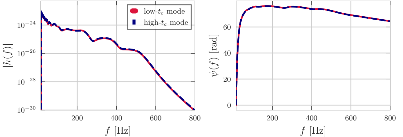
Figure 7. Comparison of the waveform amplitude |h(f)| and phase \psi(f) (projected onto the LIGO-Hanford detector) for the maximum likelihood samples from the low- t_c and high- t_c modes. There is considerable agreement between the two waveforms.
