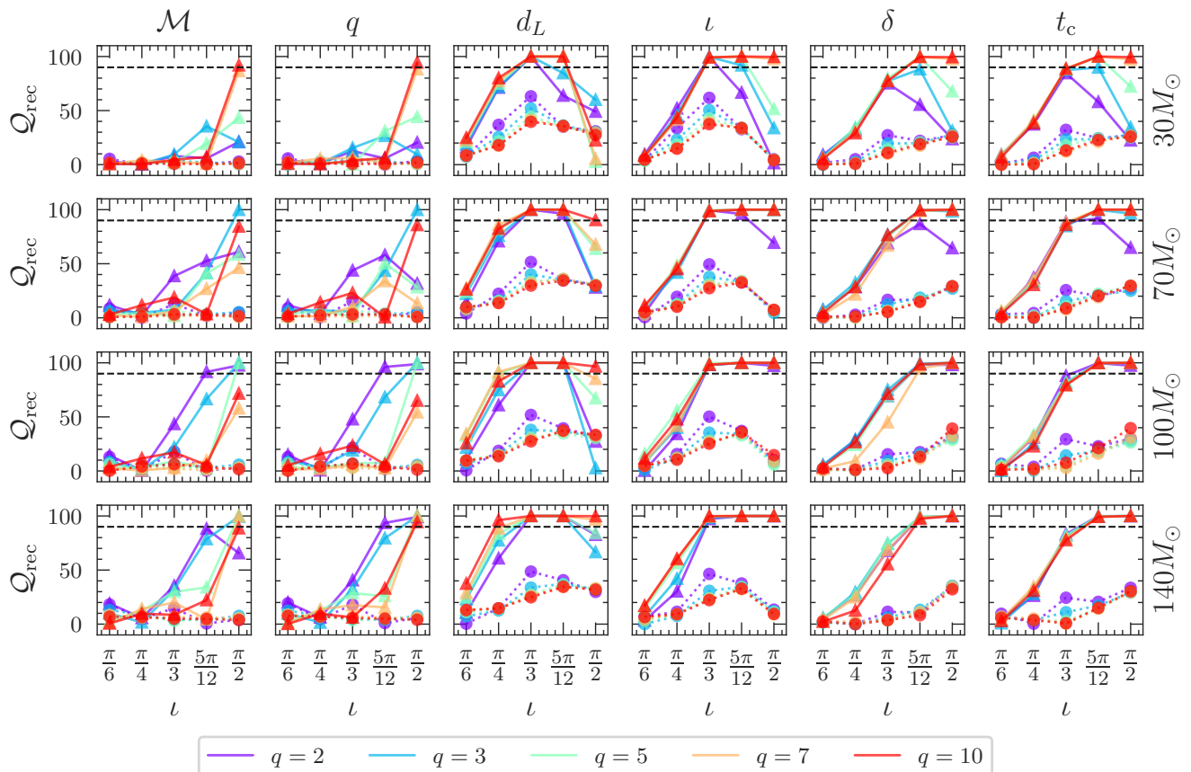
Figure 5. Same as Fig. 4 but at \rho = 50 .
