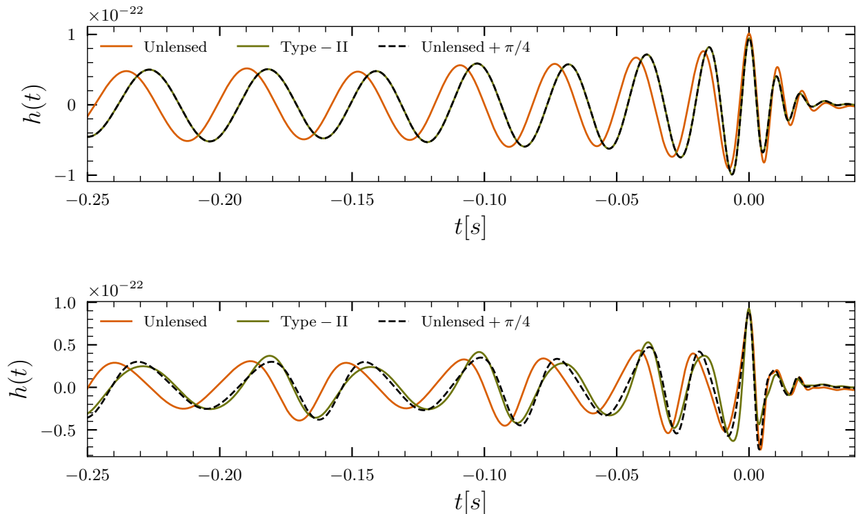
Figure 1. The unlensed signal, the Type-II signal, and the unlensed signal with a shift in the coalescence phase \phi_c by \pi/4 for the parameters M = 100M_\odot , q = 7 , \iota = 0 (top panel) and \iota = \pi/3 (bottom panel). For the zero inclination (top panel), i.e., when mainly 22 mode contributes, the GR signal reproduces the Type-II image signal very well by adjusting its coalescence phase while for high inclination (bottom), Type-II signal is not reproduced by the GR signal fully, i.e., there are additional distortions left.
