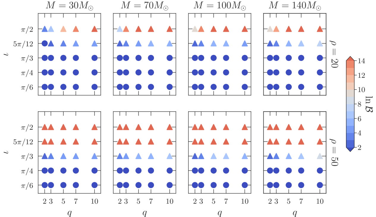
Figure 2. Type-II lensed BBH injections with a network SNRs \rho = 20 (upper row) and \rho = 50 (lower row) shown in the \iota - q plane for different total masses. The color bar shows the \ln \mathcal{B} between the Type-II and the Type-I recoveries. Injections which cross our threshold of \ln \mathcal{B} \geq 2 are plotted using triangles (i.e., distinguishable image types) while the others are plotted using circles.
