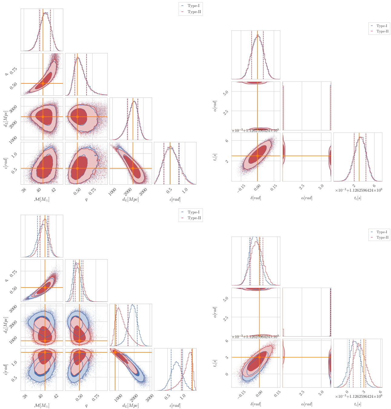
Figure 3. (Top Row) The recovery of source parameters of an injected Type-II signal using Type-I (blue) and Type-II (red) templates for q = 2 , M = 100M_{\odot} , \rho = 20 , and \iota = \pi/6 . The plots show recovery of chirp mass \mathcal{M} , mass ratio q , luminosity distance d_L , inclination \iota , sky locations \delta (dec) and \alpha (RA), and time of arrival t_c in the geocenter frame. The orange lines show the injected value. There is no appreciable difference between the posterior distributions for both the recoveries due to the low inclination and small SNR in the higher modes. (Bottom Row) The recovery of source parameters of an injected Type-I signal using Type-I (blue) and Type-II (red) templates for q = 2 , M = 100M_{\odot} , \rho = 20 , and \iota = 5\pi/12 . There is now a bias in the inclination and the distance, and the injected value is not recovered within 1\sigma . The bias in the distance also biases the recovery of the source frame masses. There are also some insignificant biases in the recovery of the sky locations and time of arrival.
