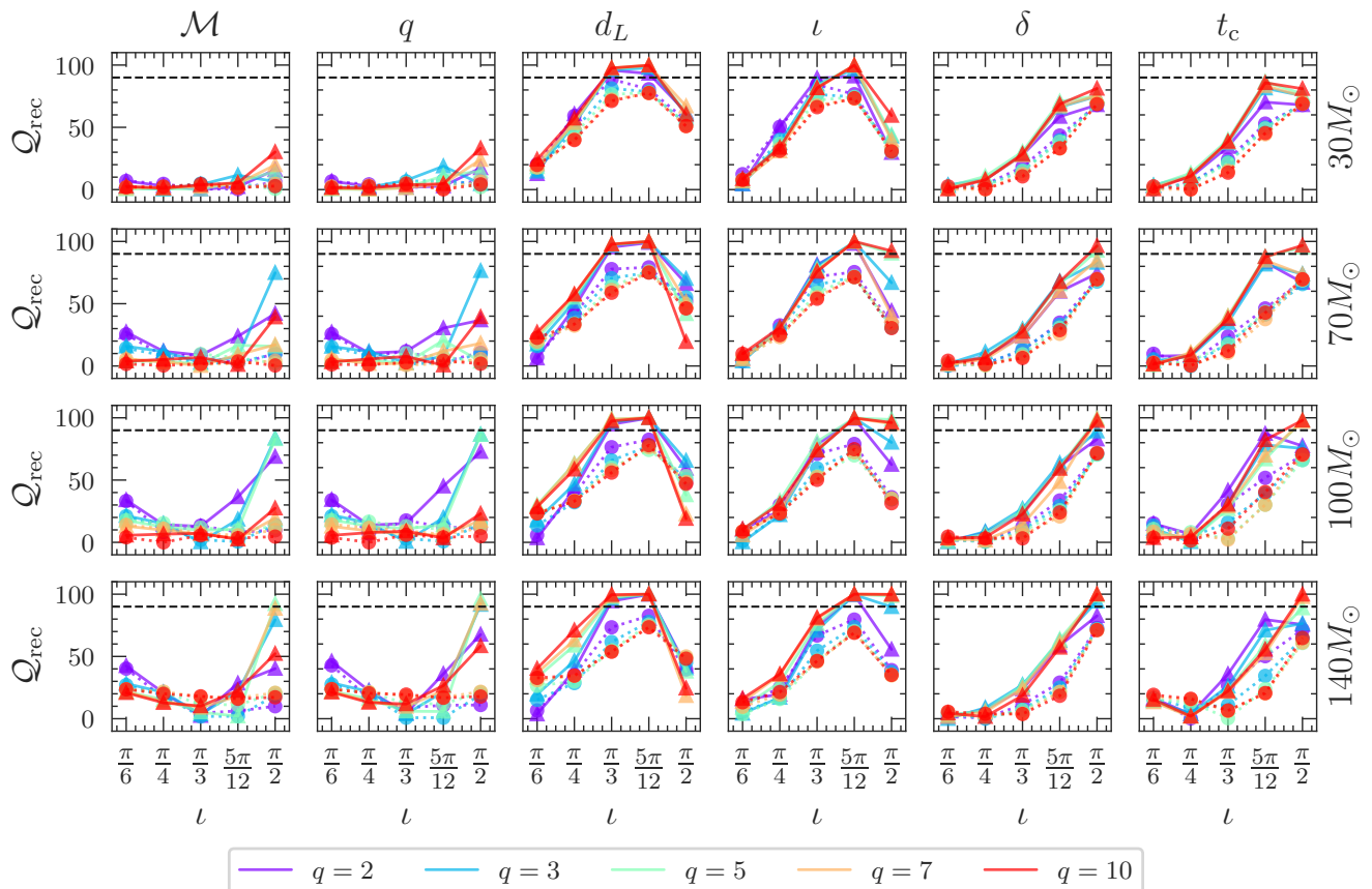
Figure 4. Each panel shows the quantiles ( Q_{\text{rec}} ) of the injection value recoveries against the inclination angle ( \iota ) of the injected BBH systems for a given total mass ( M ) (labeled on the right side of the panel) and SNR \rho = 20 . The injections are the Type-II lensed nonspinning BBH signals and the recoveries are with the Type-I template (solid lines) and the Type-II template (dashed lines), accounting for the additional phase shift of \pi/4 . At the top of the first panel, we label the parameters of the BBH systems that we are interested in. In each plot, the different colors denote the different mass ratios of the BBH systems. A lower quantile value denotes a more accurate inference of a parameter. The anomalous dips in Q_{\text{rec}} at high values of \iota are due to bimodalities in the recovery of t_c , \iota and \delta at these values. We investigate these further in Appendix A.
