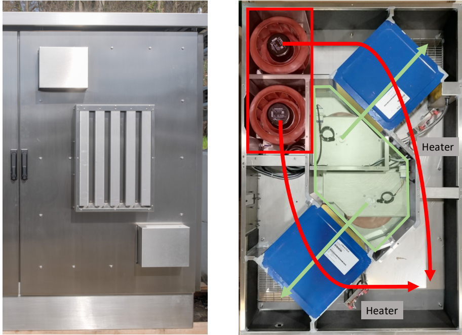
Figure 52 Left: Front view of the Häwa outdoor cabinet with the prototype air-to-air heat exchanger installed in the right door. Right: Inside view of the air-to-air heat exchanger (120 cm x 80 cm) with two redundant circuits. The inlet air from the outside goes from the middle of the device through the two heat exchanger to the lower left and upper right corner to the air outlets. Each heat exchanger has orthogonal air flow and keeps the inner circuit separate from the outer circuit. The air to be cooled from inside of the cabinet flows through the heat exchanger from the top left to the outlet into the cabinet at the bottom right.
