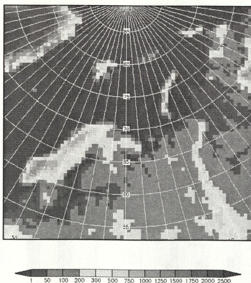
Figure 1: Model region of the Barents Sea, Orography [m].
