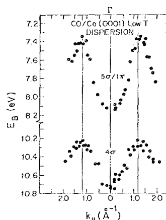
FIG. 3. Dispersion results for low temperature phase.
