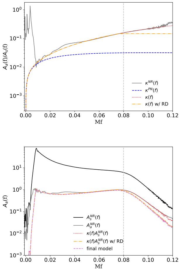
FIG. 8: The amplitude ratio (top) and amplitude (bottom) for the ( q = 2, \chi = 0.4, \theta_{LS} = 90^\circ ) configuration. The vertical line indicates the ringdown frequency for the ( \ell = 2, |m| = 2 ) multipoles.
