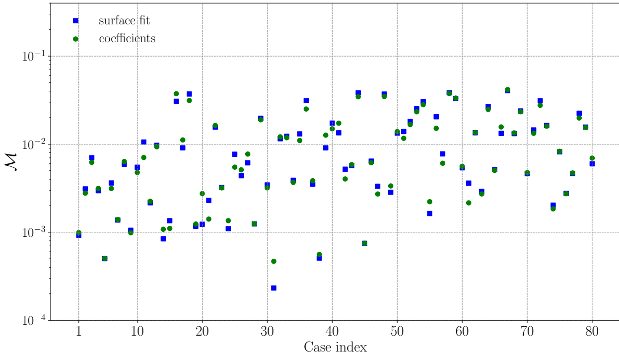
FIG. 14: Mismatches (same as Fig. 13) showing comparison of the amplitude model constructed using the spin magnitude-independent surface fit of Eq. (16) ( blue squares ) with the amplitude model constructed from the true fit coefficients ( green circles ).
