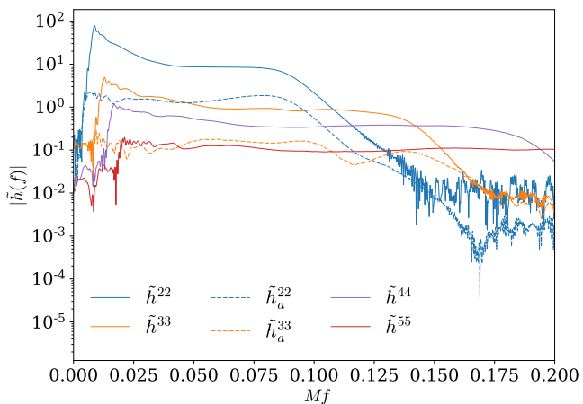
FIG. 1: Frequency-domain amplitude of co-precessing-frame symmetric and anti-symmetric contributions for a ( q = 2, \chi = 0.8, \theta_{LS} = 90^\circ ) configuration. The figure shows the symmetric contributions to (2, 2), (3, 3), (4, 4) and (5, 5), and the anti-symmetric contributions to (2, 2) and (3, 3).
