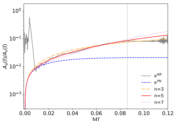
FIG. 5: Amplitude ratio for the ( q = 1, \chi = 0.4, \theta_{LS} = 60^\circ ) configuration, for the NR data, the PN ratio \kappa_{\text{PN}} , and fits to higher-order corrections as in Eq. (16), with n = 3, 5, 7 . The vertical dashed line indicates the ringdown frequency.
