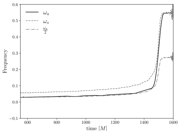
FIG. 3: The symmetric and anti-symmetric frequencies obtained from NR data of a ( q = 2, \chi = 0.7, \theta_{LS} = 90^\circ ) configuration. During inspiral the anti-symmetric frequency, \omega_a , is about half of the symmetric frequency, \omega_s (or nearly equal to the orbital frequency), and close to merger quickly catches up with the symmetric frequency. As expected from perturbation theory, \omega_s = \omega_a during ringdown.
