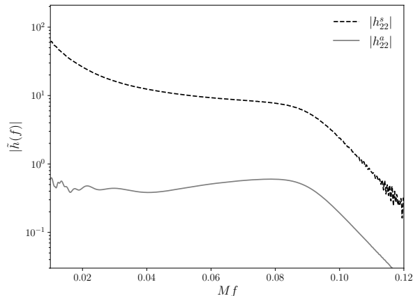
FIG. 4: The amplitude of the ( l = 2, m = 2 ) symmetric and anti-symmetric waveform components in the frequency-domain co-processing frame for a ( q = 1, \chi_1 = 0.4, \theta_{LS} = 60^\circ ) NR simulation.
