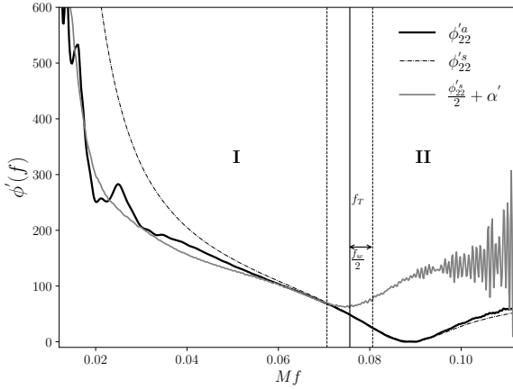
FIG. 11: The anti-symmetric phase derivative (thick black line), the symmetric phase derivative (grey dashed line) and the combination of half of the symmetric phase derivative with the derivative of the precession angle \alpha (thin grey line). The specific configuration shown here is for a single-spin binary with ( q = 1, \chi = 0.2, \theta_{LS} = 30^\circ ).
