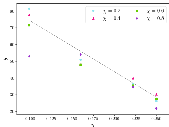
FIG. 10: The b coefficient as a function of the symmetric mass ratio, \eta , for a selected angle \theta_{LS} = 90^\circ and all the available spin values, \chi = [0.2, 0.4, 0.6, 0.8] . The grey line shows the surface fit, b(\eta, 90^\circ) from Eq. (18).
