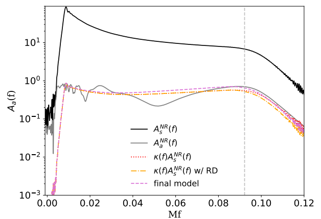
FIG. 7: The amplitude ratio (top) and amplitude (bottom) for the ( q = 1, \chi = 0.8, \theta_{LS} = 30^\circ ) configuration. The vertical line indicates the ringdown frequency for the ( \ell = 2, |m| = 2 ) multipoles.
