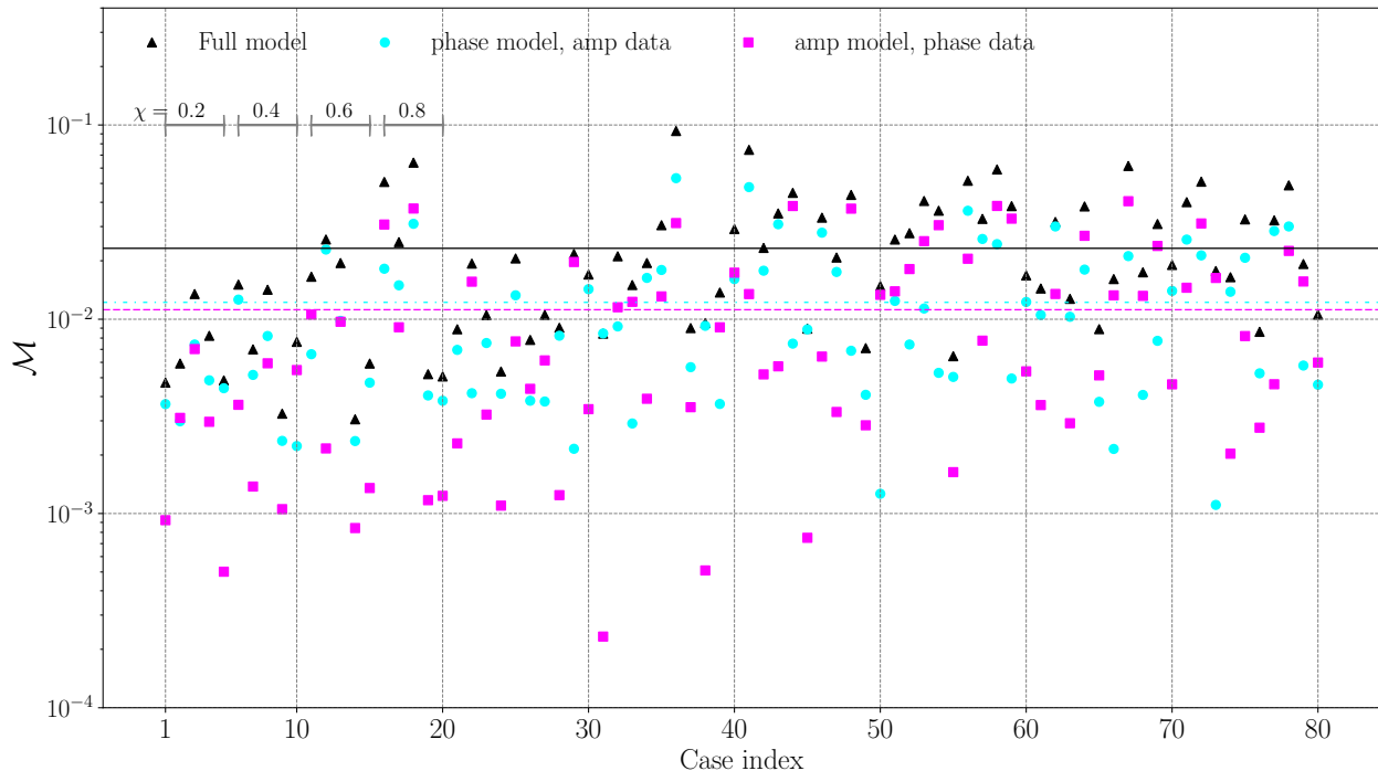
FIG. 13: Mismatches of the anti-symmetric waveform model in the co-processing frame with NR data. The black triangles show the mismatches for the combined amplitude and phase model while the magenta squares (cyan circles) show the mismatches for just the amplitude (phase) model with the phase (amplitude) constructed from NR data. The dashed magenta and cyan lines show the average mismatch for the amplitude and phase model, respectively; on average they are of comparable accuracy. The black solid line shows the average mismatch for the overall model. The x -axis denotes the case index of the NR simulation as usual i.e., five different \theta_{LS} for each spin magnitude shown in figure, for q = 1, 2, 4 and 8 .
