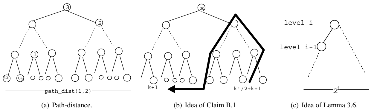
Figure 5: (a) Path distance between 1 and 2 is the number of leaves in the subtree rooted at 3, the lowest common ancestor of 1 and 2. (b) For one unscratched left breakpoint, k'/2 + k + 1 to be combined with another right breakpoint k + 1 on the left, k'/2 + k + 1 has to be carried to L by some intervals. Moreover, one interval can carry at most two unscratched breakpoints at a time. (c) Sending a message between nodes on level i and i - 1 can increase the covered path distance by at most 2^i .
