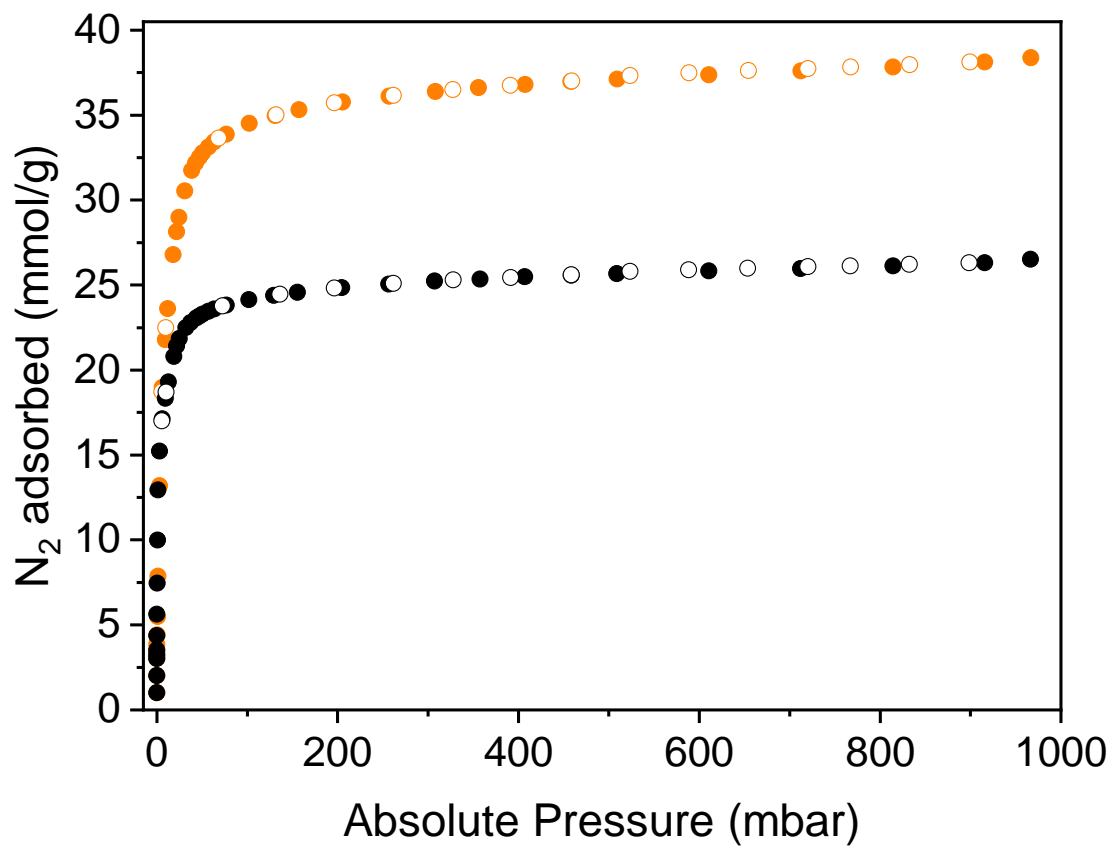
Fig. S5. Nitrogen adsorption (filled symbols) and desorption (open symbols) isotherms collected at 77 K for \text{Fe}_{1.8}\text{Zn}_{3.2}\text{Cl}_4(\text{btdd})_3 (orange) and \text{Fe}_{1.8}\text{Zn}_{3.2}(\text{prv})_4(\text{btdd})_3 (black).
