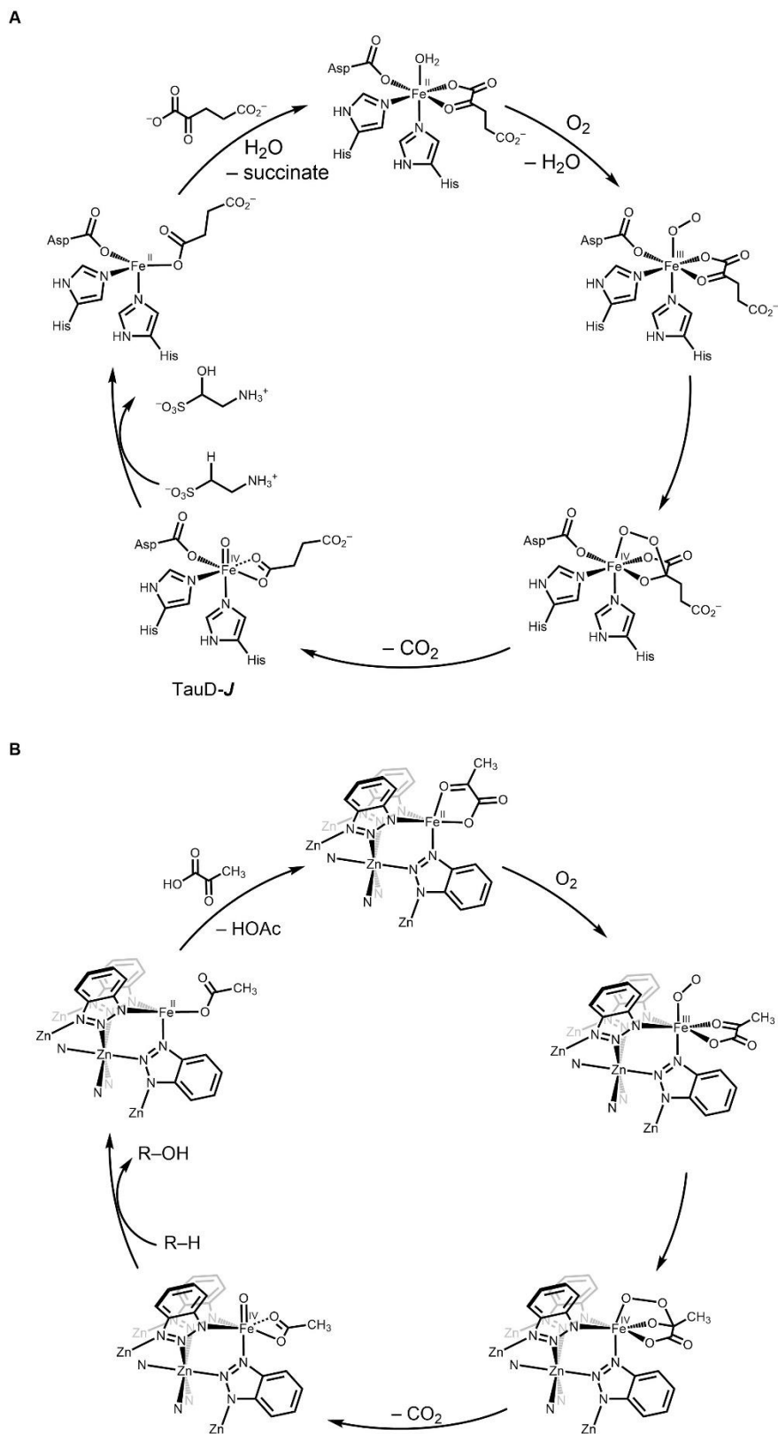
Fig. S71. (A) Catalytic cycle for taurine C–H hydroxylation by TauD. (B) Proposed catalytic cycle for C–H hydroxylation by FeZn 4 (prv) 4 (btdd) 3 .
