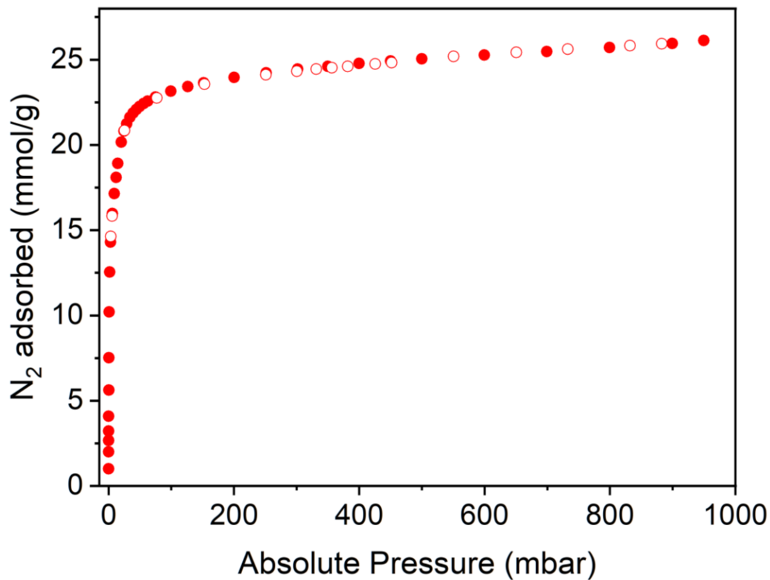
Fig. S28. Nitrogen adsorption (filled symbols) and desorption (open symbols) data collected at 77 K for \text{FeZn}_4(\text{moba})_4(\text{btdd})_3 . The BET surface area is 2180 \pm 11 \text{ m}^2/\text{g} .
