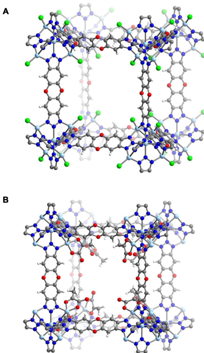
Fig. S15. Structures of Zn_5Cl_4(btdd)_3 ( A ) and Zn_5(prv)_4(btdd)_3 ( B ) obtained from single-crystal x-ray diffraction. Average positions of the linker atoms are shown because of disorder. Light blue, lime green, gray, red, blue, and white spheres represent Zn, Cl, C, O, N, and H atoms, respectively.
