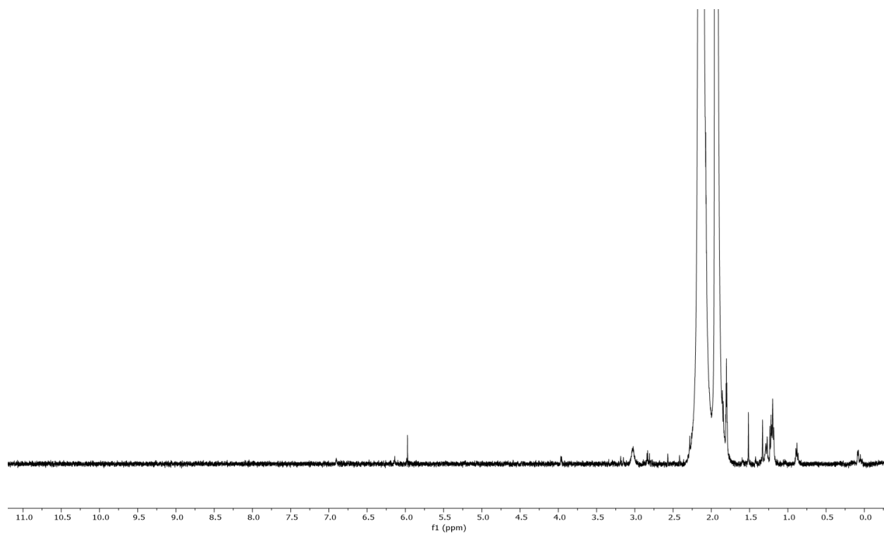
Fig. S69. Proton NMR spectrum (500 MHz, \text{CD}_3\text{CN} , 25 °C) of \text{Fe}_{1.8}\text{Zn}_{3.2}(\text{prv})_4(\text{btdd})_3 exposed to air and extracted with \text{CD}_3\text{CN} . No ethanol is present.
