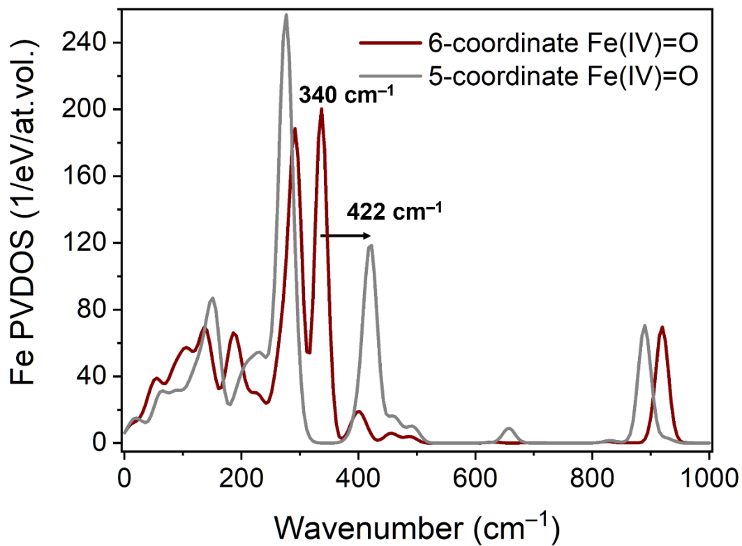
Fig. S46. Density functional theory-computed NRVS iron PVDOS distributions for \text{Fe(O)}(\kappa^1\text{-OAc})\text{Zn}_4(\text{prv})_3(\text{bta})_6 (gray) and \text{Fe(O)}(\kappa^2\text{-OAc})\text{Zn}_4(\text{prv})_3(\text{bta})_6 (dark red).
