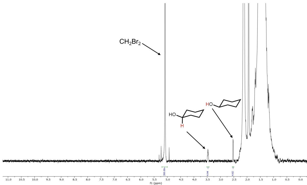
Fig. S52. Proton NMR spectrum (600 MHz, CD 3 CN, 25 °C) of the solution resulting from the stoichiometric reaction of FeZn 4 (prv) 4 (btdd) 3 with O 2 and cyclohexane. The yield determined for cyclohexanol is 24%.
