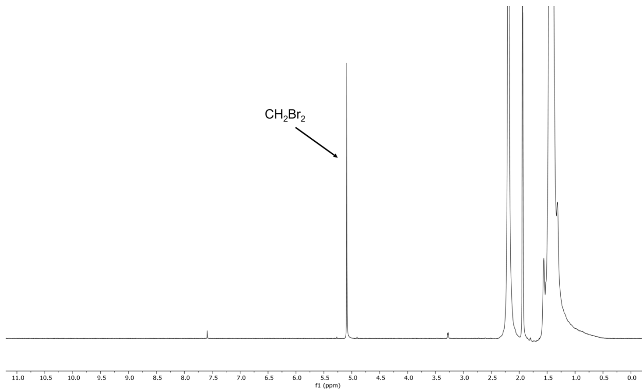
Fig. S57. Proton NMR spectrum (500 MHz, CD 3 CN, 25 °C) of the supernatant resulting from the stoichiometric control reaction between FeZn 4 Cl 4 (btdd) 3 dosed in situ with O 2 and cyclohexane. No cyclohexanol or cyclohexanone was detected.
