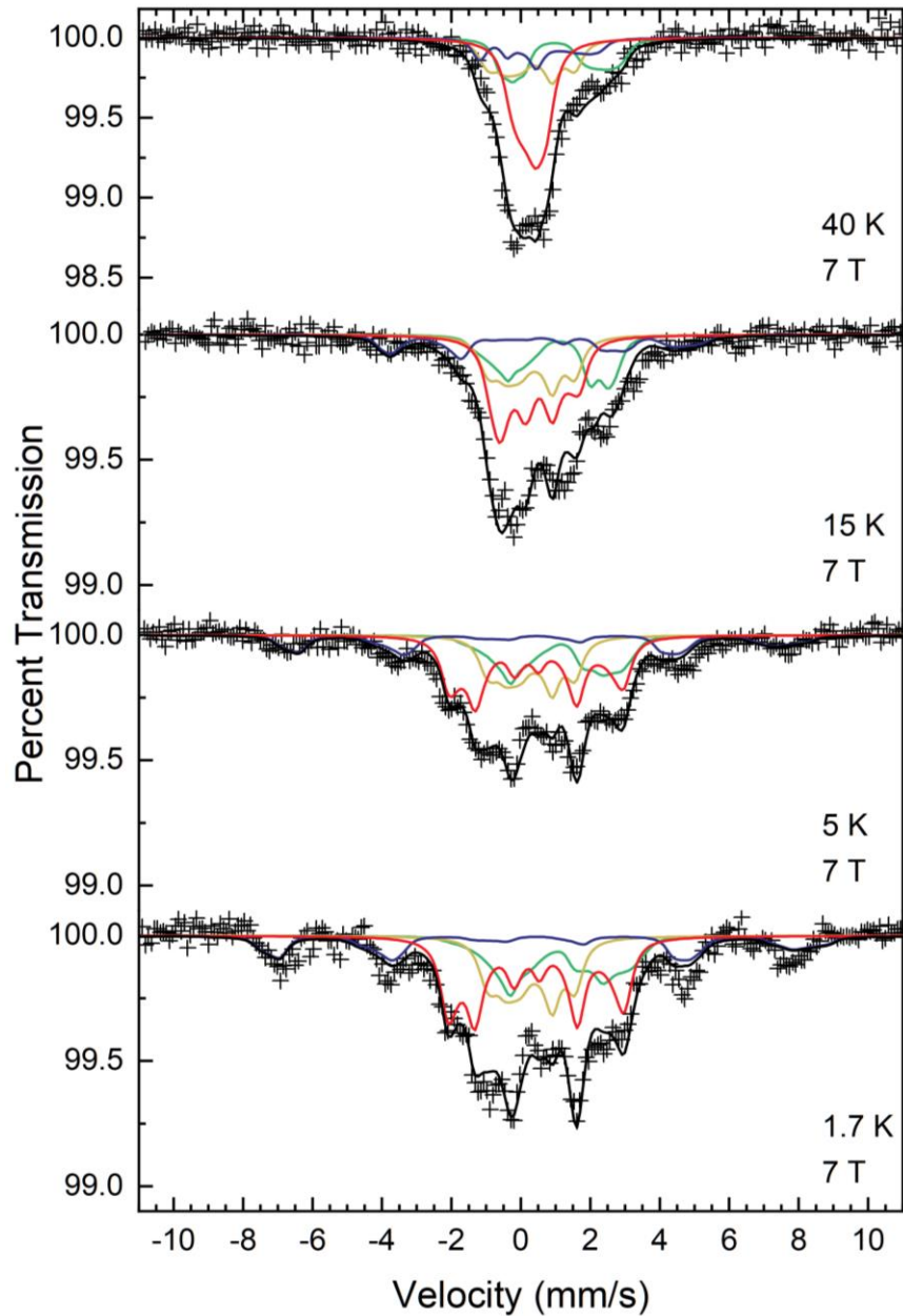
Fig. S34. Mössbauer data collected for \text{O}_2 -dosed \text{FeZn}_4(\text{moba})_4(\text{btdd})_3 at 40, 15, 5, and 1.7 K and 7 T (plus symbols) plotted together with the optimized model for a system featuring S = 1 \text{Fe(IV)=O} species, as discussed in Section 2.12.3 (solid black line). The four subspectra (modeled with the spin Hamiltonian parameters reported in table S14) correspond to the following species in the framework: S = 2 \text{Fe(II)} species (green); S = 5/2 \text{Fe(III)} species (blue); S = 1 \text{Fe(IV)=O} species (red); S_{\text{tot}} = 0 species formed from antiferromagnetic coupling between neighboring S = 1 \text{Fe(IV)=O} sites in one cluster node (dark yellow).
