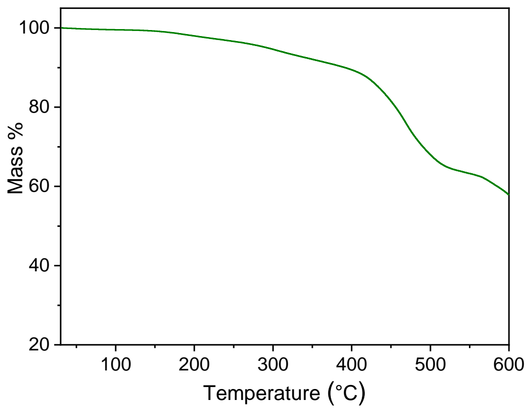
Fig. S7. Thermogravimetric analysis data for FeZn 4 (prv) 4 (btdd) 3 .
