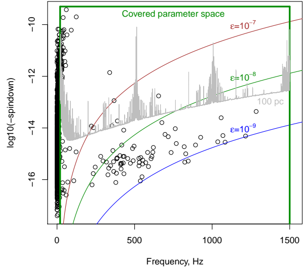
FIG. 1. This plot shows the expected gravitational wave frequency and frequency-derivative of isolated neutron stars from the ATNF catalog [33] (circles). The curves show the frequency/frequency-derivative combinations for a gravitar (a neutron star losing energy solely due to gravitational wave emission) for different values of the ellipticity. Following [34] we observe that known pulsars have spin-down values that lie at or above the curve \epsilon = 10^{-9} . For gravitars this would imply that the minimum ellipticity is around 10^{-9} . The region above the grey trace and enclosed by the box of green straight lines shows the frequency/frequency-derivative combinations of optimally oriented gravitars at 100 pc, that our search could detect. The frequency-derivative of a detectable gravitar is proportional to the square of the distance, so if the distance increases by a factor of 10, correspondingly the grey trace moves up by a factor of 100.
