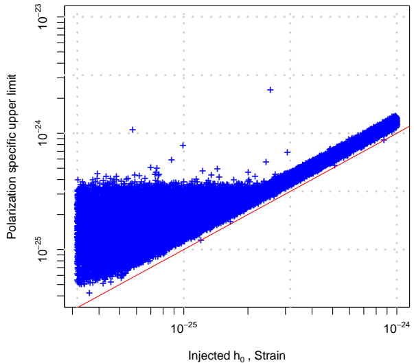
FIG. 4. Polarization-specific upper limits versus injected strain for a set of more than 31000 software injections. The upper limits are computed using \iota and \psi of the injected signals.
