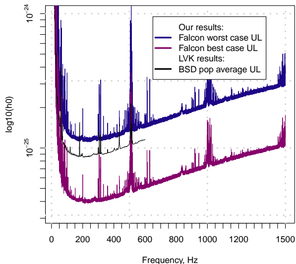
FIG. 7. This plot shows upper limits similar to those shown in Figure 2, but for the location of G189.1+3.0. Latest LIGO/Virgo/KAGRA results [32] are shown for comparison. The LVK upper limit curve was computed as minimum of Hanford, Livingston and Virgo data.
