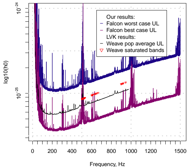
FIG. 6. This plot shows upper limits similar to those shown in Figure 2, but for the location of Vela Jr. Latest LIGO/Virgo/KAGRA results [31] are shown for comparison. The triangles mark saturated bands for which the Weave results are invalid.
