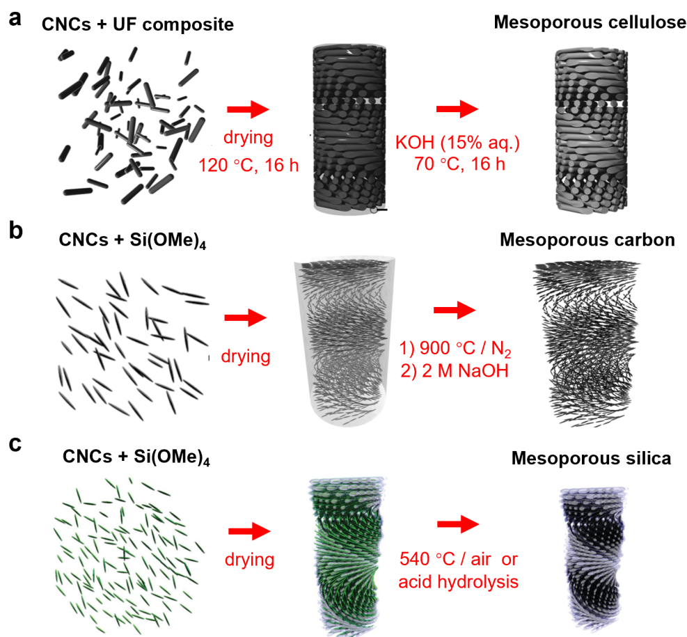
Figure 90. Fabrication of mesoporous helicoidal materials via the selective removal of specific components from a cholesteric CNC composite. (a) CNC and urea formaldehyde (UF) composites were heat treated and then exposed to strong base, leading to mesoporous cellulose films. Adapted with permission from ref 790. Copyright 2014 John Wiley and Sons. (b) CNC and TMOs composites were pyrolyzed at high temperature under nitrogen atmosphere and then exposed to strong base to remove the silica, resulting in mesoporous carbon films. Adapted with permission from ref 781. Copyright 2011 John Wiley and Sons. (c) Alternatively, the same initial composites were exposed to high temperature or strong acid to selectively remove the cellulose, leading to mesoporous silica films. Adapted with permission from ref 800. Copyright 2013 John Wiley and Sons.
