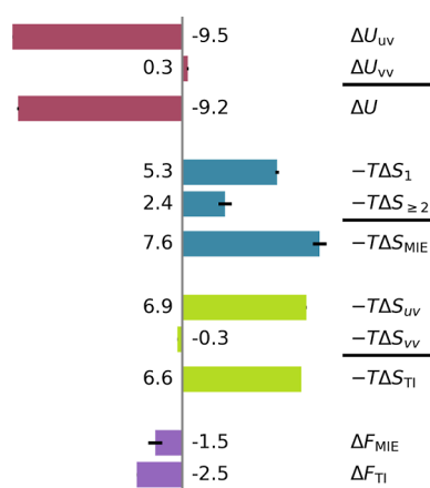
Figure 3. Solvation free energy contributions (in kJ mol -1 ) of the fixed Lennard-Jones solute in an argon-type liquid. Red bars denote the internal energy change and its contributions. Colors correspond to those in Figure 2; blue and green bars denote the entropy change and its contributions, calculated using PerIMut and TI, respectively. Purple bars show the overall free energy change, as calculated using PerIMut and TI. Estimated sampling uncertainties are shown as small black bars. Within each colored group, the lowest bar is the sum of the upper 2 bars, as indicated by the horizontal black summation lines.
