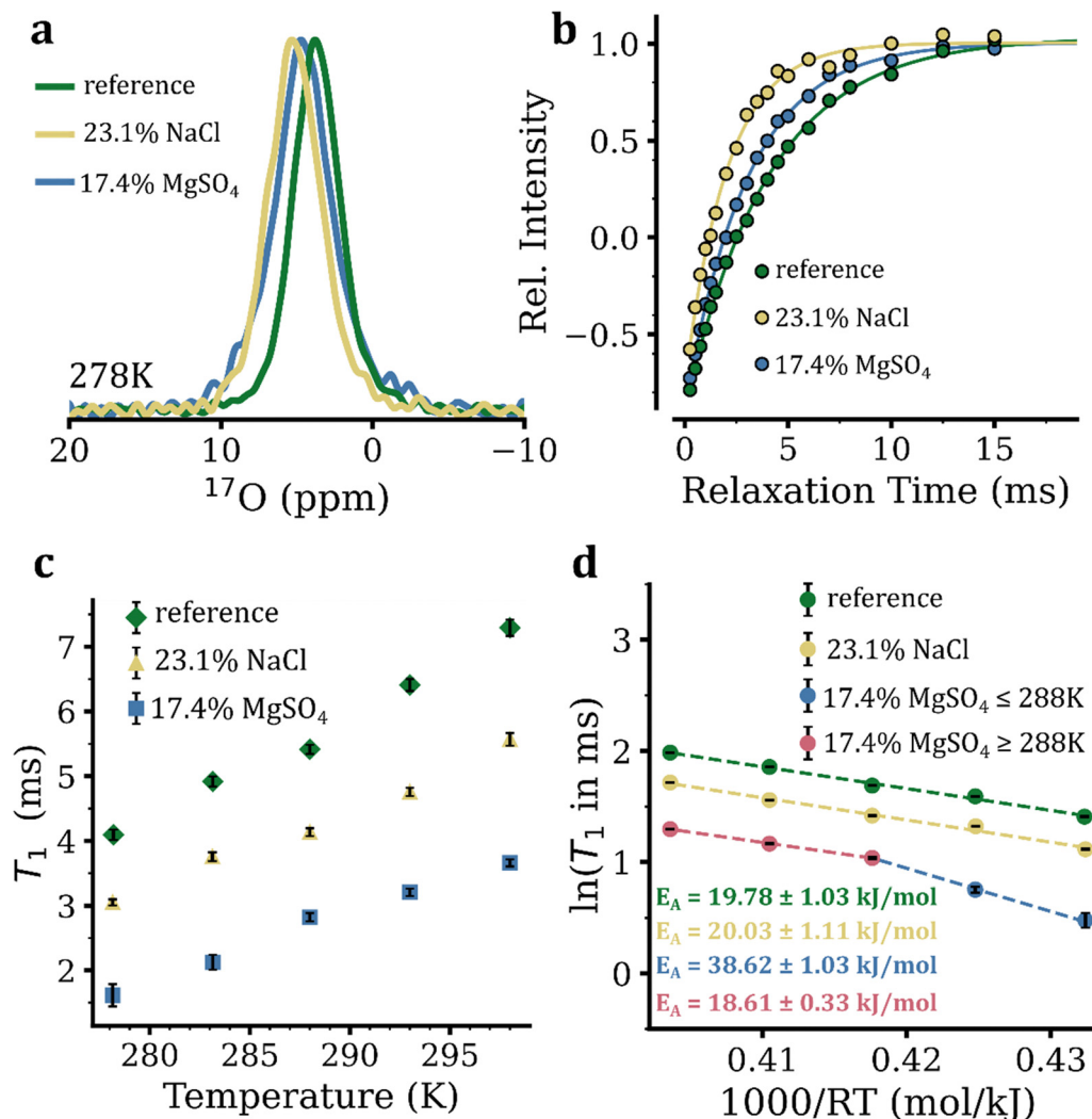
Fig. 2 Water mobility in reference (pure water) and eutectic NaCl and MgSO 4 solutions probed through 17 O longitudinal spin–lattice ( T 1 ) relaxation times. (a), (b) 1D 17 O NMR spectra and inversion-recovery data of the mentioned samples shown as an example for the temperature of 5 °C. (c) 17 O T 1 relaxation times, shown as a function of temperature in the range 278–298 K. The 17 O T 1 relaxation times of water is the smallest in MgSO 4 solution, followed by the NaCl solution. (d) Arrhenius analysis of the temperature dependence of 17 O T 1 relaxation times. The slopes of the fitted lines represent the (apparent) activation energies ( E A ) for the rotational mobility of water molecules. The error bars shown in the different panels were derived from the standard error of the least-squares curve fitting and in some cases were smaller than the symbol size.
