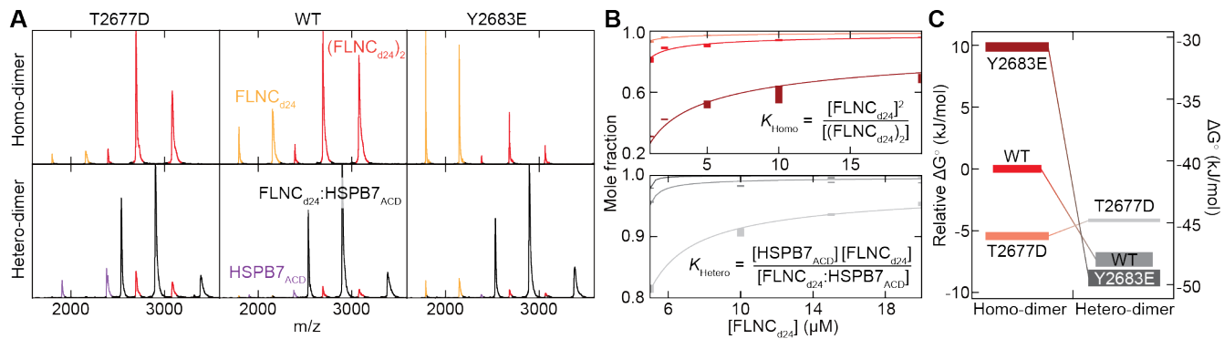
Fig. 4 | Mimicking phosphorylation at T2677 and Y2683 has opposite effects in modulating
