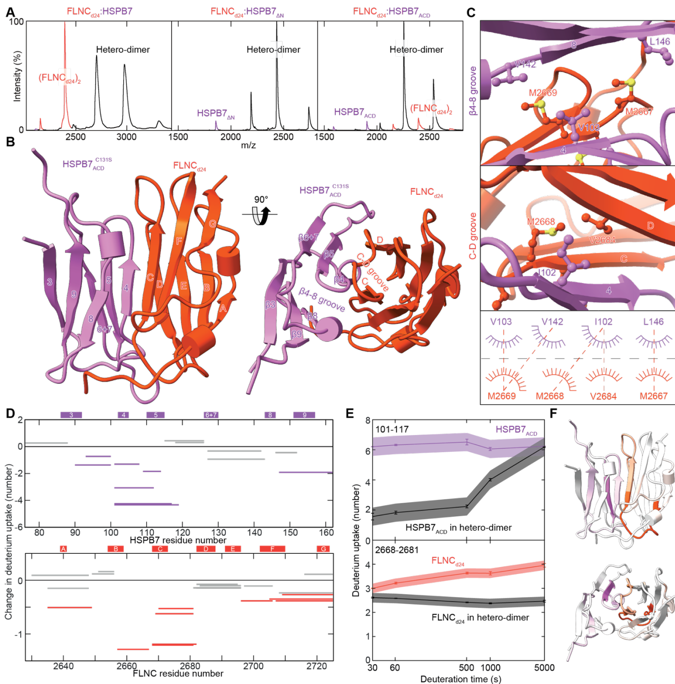
Fig. 3 | Hetero-dimerisation of HSPB7 and FLNC. A Native MS experiments show that FLNC d24 (red) forms hetero-dimers (black) with HSPB7, HSPB7 ΔN and HSPB7 ACD (purple). No complexes between the FLNC d24 homo-dimer and HSPB7 are observed, revealing how homo- and hetero-dimerisation are directly competitive. Proteins were mixed at a monomer ratio of 1:1, but the instability of full length HSPB7 means it was somewhat depleted in solution such that FLNC d24 was effectively
