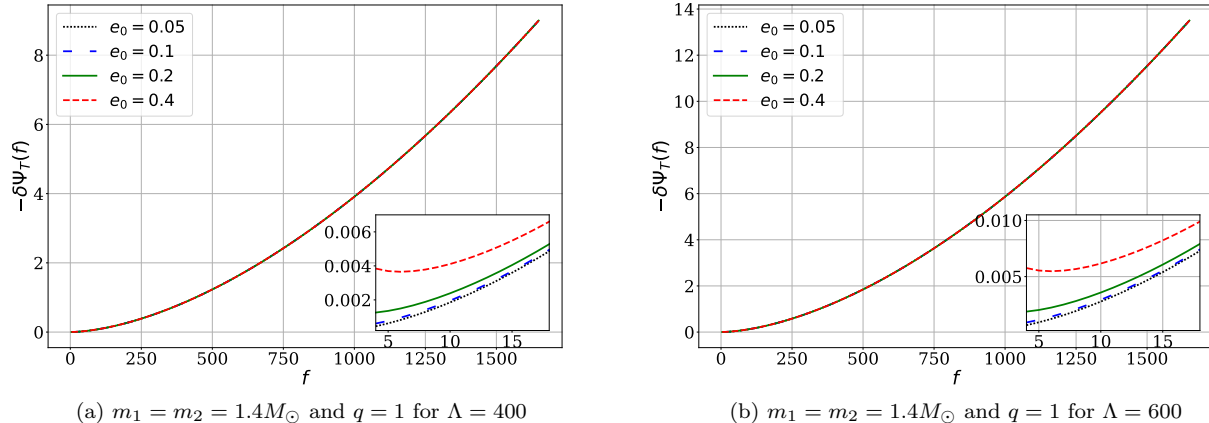
FIG. 2. We show the total tidal phasing -\delta\Psi_T (in radian) for a binary with two 1.4M_\odot neutron stars as a function of gravitational wave frequency f in the range f_i = 4\text{Hz} to f_{ISCO} . The initial eccentricities taken for the figure are e_0 = 0.05, 0.1, 0.2, and 0.4 with \Lambda_1 = \Lambda_2 = \Lambda = 400 and 600 respectively.
