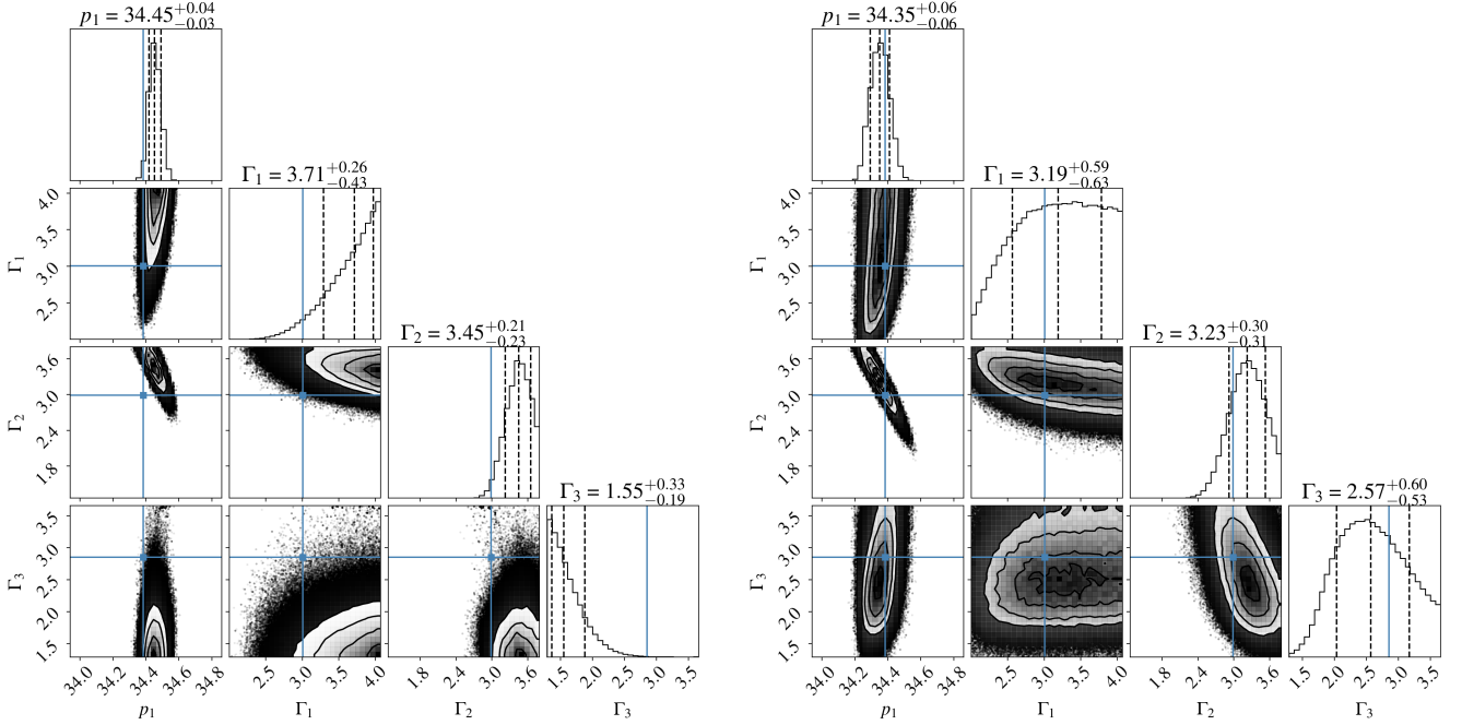
FIG. 11. Same as Fig. 10 but for observations of moderately rotating neutron stars as shown in Tab. IV. At rotation rates of 350 – 550 Hz or axis ratios of \tau \approx 0.96 - 0.97 , the stars' oblateness is no longer negligible and we observe a strong bias in the posteriors, in particular for \Gamma_1 and \Gamma_3 , when using the old framework. The new framework reconstructs the PPA parameters well.
