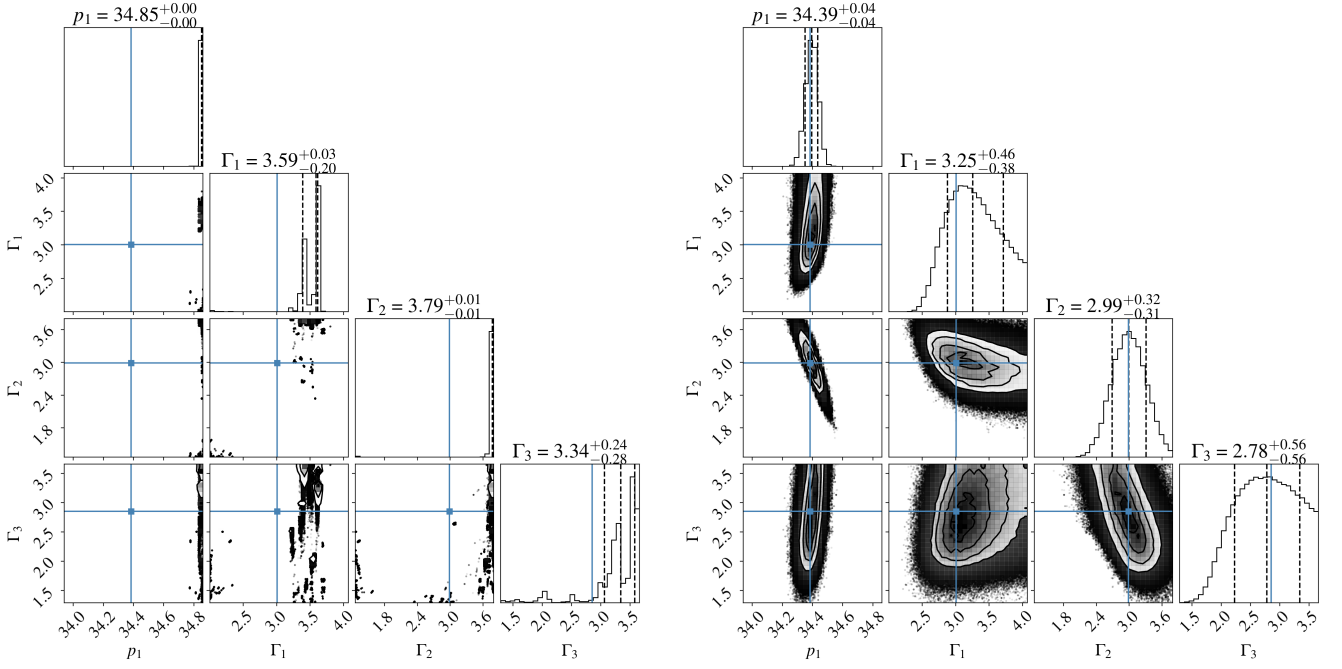
FIG. 12. Same as Fig. 10 but for observations of rapidly rotating neutron stars as shown in Tab. V. With axis ratios of \tau \approx 0.73 - 0.90 , the stars are far from sphericity and as a result, the old framework fails completely. The new framework built on the universal relations for rapid rotation, again, yields very useful results.
