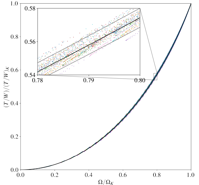
FIG. 5. A scatter plot of the rescaled (T/W)_n against the fractional angular rotation rate \Omega_n for the 1550 sequences in our dataset. An inset shows a zoom-in onto a small region of the graph; almost all data points are inside a very narrow band (with less than 1% relative error which is indicated by grey lines) around the polynomial fit (black solid line). The few individually visible points outside the dense band have a relative error of less than 2%.
