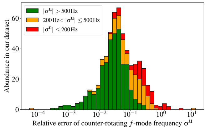
FIG. 8. A stacked histogram of the relative errors as defined in Eq. (8) when estimating the counter-rotating f -mode frequency using Eq. (7). Since relative errors for low frequencies are an unreliable measure for accuracy, we split the set of relative errors into three groups depending on the absolute value of the f -mode frequency. When the magnitude of the f -mode is larger than 500 Hz (shown in green), the relative errors peak at 3% and are larger than 10% only in a few cases. For smaller magnitudes of the f -mode frequency (shown in orange and red), the relative error naturally increases. However, there are still many instances where even low-frequency f -modes are estimated with only a small relative error.
