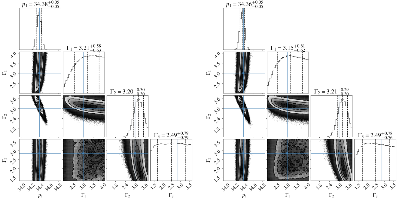
FIG. 10. Results of the MCMC analysis using observations of slowly rotating neutron stars listed in Tab. III as described in the main text. The two corner plots compare the results using the old framework with slow-rotation approximations (left panel) and the new framework based on universal relations that allow rapid rotation (right panel). The blue lines indicate the injected EOS parameters and black dashed intervals define the [0.16, 0.84] quantils. The results of both frameworks are almost identical which reconfirms that the slow-rotation approximation is justified for observations of neutron stars that rotate sufficiently slowly (cf. Ref. [38]).
