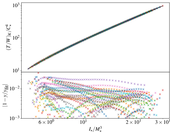
FIG. 6. The scaled value of T/W of neutron stars at the Kepler limit against the mass-scaled moment of inertia of the non-rotating neutron star with the same central energy density as the rotating stars. The bottom panel shows the relative errors of the data points; the maximum relative deviation from the best fit is 3.2%.
