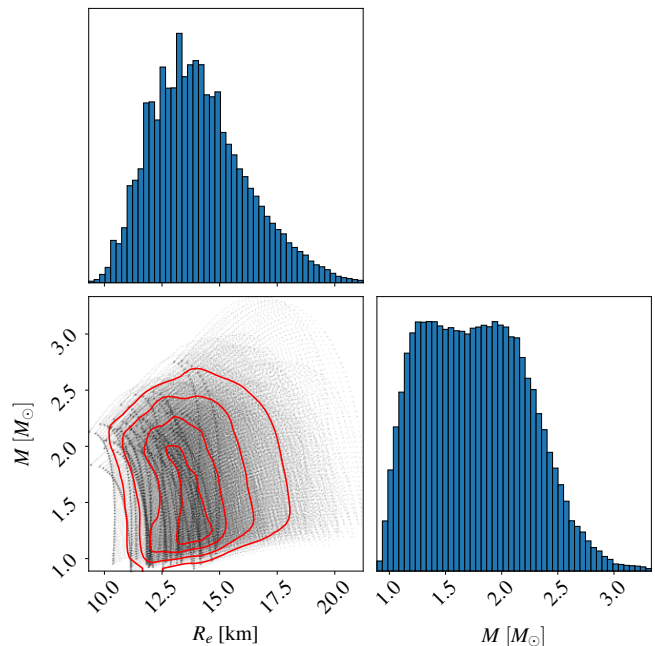
FIG. 1. A corner plot of the data set on which we construct the universal relations. Each black dot in the M vs. R diagram represents one of 83011 NS models in our dataset. Their density distribution is indicated by the red contour lines. The top and right diagram show the corresponding histograms of radius and mass, respectively.
