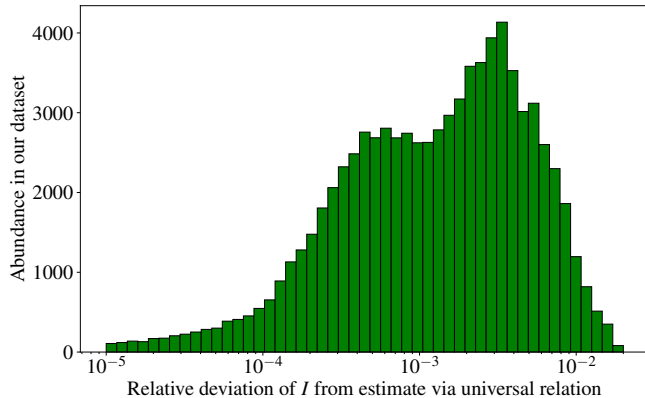
FIG. 3. A histogram of the relative deviations of our 83011 data points from the universal relation Eq. (2). The majority of data points (roughly 80%) deviate less than 0.4% from the fit and the maximum relative error is 1.9%.
