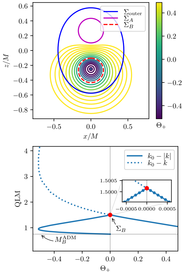
FIG. 6. Upper panel: CESs near the individual MOTS \Sigma_B in BL data with m_A = m_B = d = 1/2 . Lower panel: QLM calculated for these CESs. The inset shows a close-up near \Theta_+ = 0 . As in Fig. 5, the dotted line shows (11) calculated via \frac{1}{8\pi} \int_{\Sigma} k_0 - k . The QLM asymptotes to the ADM mass 3/4 of the end at x_B as the family approaches the puncture x_B .
