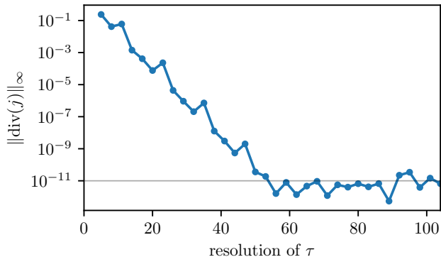
FIG. 2. Maximum residual of the OEE (6) as the resolution of our representation of \tau is increased. The error drops exponentially up to reaching a numerical roundoff at about 10^{-11} . The case shown here is for a CES with \Theta_+ \approx 0.114 in a non-time-symmetric slice.
