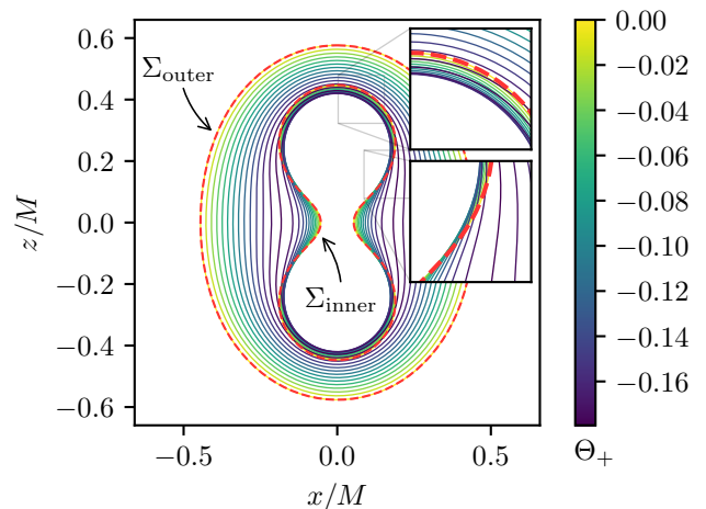
FIG. 7. Family of CESs interpolating between \Sigma_{\text{outer}} and \Sigma_{\text{inner}} in BL data with parameters m_A = m_B = d = 1/2 . Close to \Sigma_{\text{inner}} , members of this family intersect each other and hence fails to foliate the space in this interior region.
