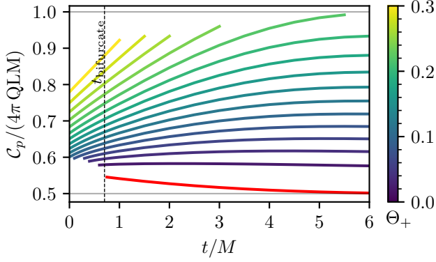
FIG. 13. Exploring the use of the Wang-Yau QLM in the hoop conjecture for the formation of the common horizon. The figure shows the ratio C_p/(4\pi \times \text{QLM}) as functions of time for various constant expansion surfaces. The curve in red refers to the common horizon while the other curves refer to positive values of the expansion; the color scale indicates the values of the expansion, which lie apart by 0.02 at the color scale's ticks. The time labeled as t_{\text{bifurcate}} is when the common horizon is formed.
