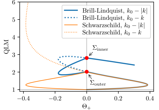
FIG. 5. Same as Fig. 3, but continuing the families to the inside of the apparent horizon in both the BL data (blue) and in a Schwarzschild slice (orange). We show a comparison of the Brown-York mass (11) calculated either via \frac{1}{8\pi} \int_\Sigma k_0 - |k| (solid lines) or via \frac{1}{8\pi} \int_\Sigma k_0 - k (dotted lines). For \Theta_+ \geq 0 , the two definitions agree. In the Brill-Lindquist case, the CES family interpolates between the inner common MOTS \Sigma_{\text{inner}} and the apparent horizon \Sigma_{\text{outer}} via surfaces with \Theta_+ < 0 . However, these latter surfaces intersect each other (Fig. 7). Monotonicity in this regime can therefore not be expected. See text for discussion.
