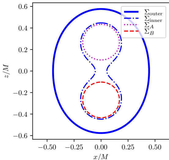
FIG. 1. Common MOTS \Sigma_{\text{outer}} , inner common MOTS \Sigma_{\text{inner}} and the two individual MOTSs \Sigma_A and \Sigma_B in Brill-Lindquist initial data with parameters m_A = m_B = d = 1/2 .
