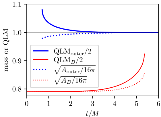
FIG. 11. QLM and area masses of \Sigma_{\text{outer}} and \Sigma_B calculated using (16) in simulation Sim1 as function of simulation time. The smaller horizon \Sigma_A (not shown) has a qualitatively similar behavior, though less pronounced, as \Sigma_B . For easier comparison, the QLM has been divided by 2 to account for the fact that for Schwarzschild, the QLM of the horizon is twice the ADM mass.
