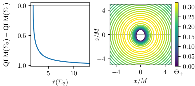
FIG. 8. Monotonicity of the QLM along a CES family going outward from \Sigma_1 = \Sigma_{\text{outer}} at time t = 2.5M in simulation Sim1. The area radius \tilde{r}(\Sigma) increases monotonically along this family. The left panel shows the difference of the QLM between \Sigma_{\text{outer}} and \Sigma_2 as \Sigma_2 is moved outward. The right panel shows the region around \Sigma_{\text{outer}} foliated by the CES family.
