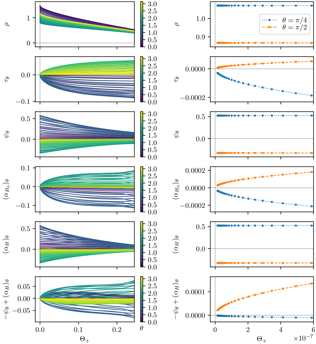
FIG. 9. Terms appearing in (9), i.e., j_\theta = \rho\tau_\theta - \psi_\theta - (\alpha_{H_0})_\theta + (\alpha_H)_\theta , where \psi = \sinh^{-1}\left(\frac{\rho\Delta\tau}{|H_0||H|}\right) . They are plotted as function of \Theta_+ for CESs outside \Sigma_{\text{outer}} . For each curve, we fix the coordinate \theta \in (0, \pi) along the surface and show its value as color. The right column is a close-up of \Theta_+ = 0 and depicts two individual values of \theta . The first five rows show the individual quantities whereas the final row shows -\psi_\theta + (\alpha_H)_\theta . The slice is from Sim1 at time t = 2.5M .
