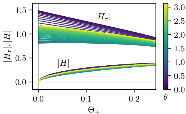
FIG. 14. Value of |H_\tau| and |H| along the CESs outside \Sigma_{\text{outer}} at simulation time t = 2.5M in Sim1. As Fig. 9, the colors indicate the coordinates on the surface.
