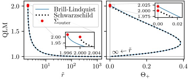
FIG. 3. QLM calculated for a family of CESs in BL data with m_A = m_B = d = 1/2 , going from spatial infinity ( \text{QLM}_\infty = 1 ) to the common horizon \Sigma_{\text{outer}} ( \text{QLM}_{\text{outer}} \approx 2.019209822 ). The dotted line shows the QLM for constant radius surfaces in the time-symmetric Schwarzschild slice for comparison. The left panel shows the QLM as function of the area radius \tilde{r} , defined by 4\pi\tilde{r}^2 = A , where A is the area, and the right panel as function of the expansion \Theta_+ .
