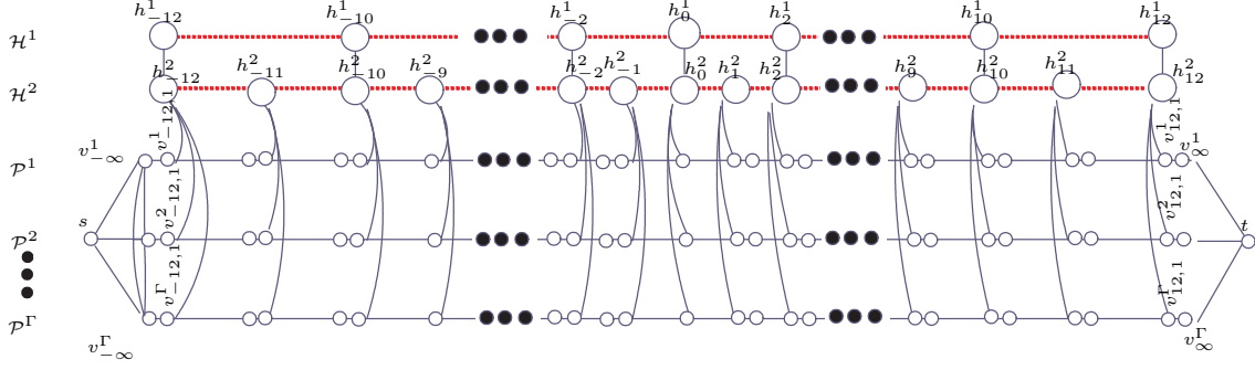
Figure 1: An example of F(\Gamma, \kappa, \Lambda) where \Lambda = 2 and 2 \leq \kappa < 3 .
