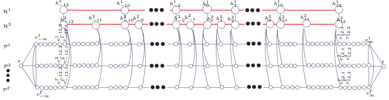
Figure 2: An example of G(\Gamma, \kappa, \Lambda) where \kappa = 2.5 and \Lambda = 2 . The dashed edges (in red) have one copy while other edges have infinitely many copies. Note that \phi'_{10} = 4 and thus there are 4 nodes in each subpath \mathcal{P}^i_{10} , for all i . Note also that \phi'_{10} is less than \phi_{10} which is 6.
