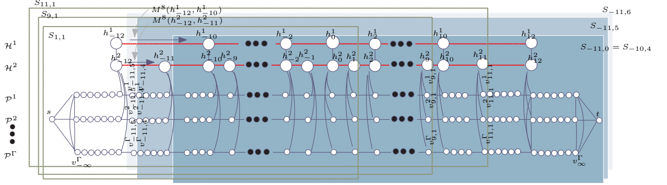
Figure 3: An example of round 11 in the proof of Theorem 2.3 (see detail in Example 2.6).
