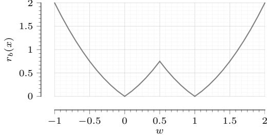
Figure 3: W -shaped regularizer. To push the weights towards a binary solution during optimization, which allows a better quantization, we employ the W -shaped regularizer discussed in the main paper (here, \lambda = \kappa = 1 ).
