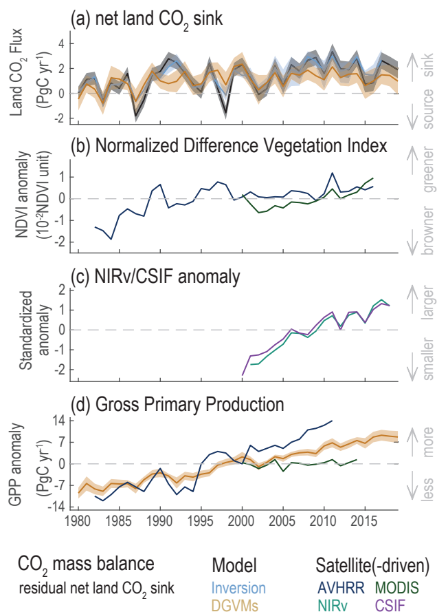
Figure 5.10 | Trends of the net land CO 2 sink and related vegetation observations during 1980–2019.
