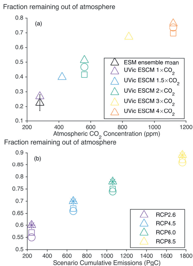
Figure 5.34 | Removal effectiveness of carbon dioxide removal (CDR).
