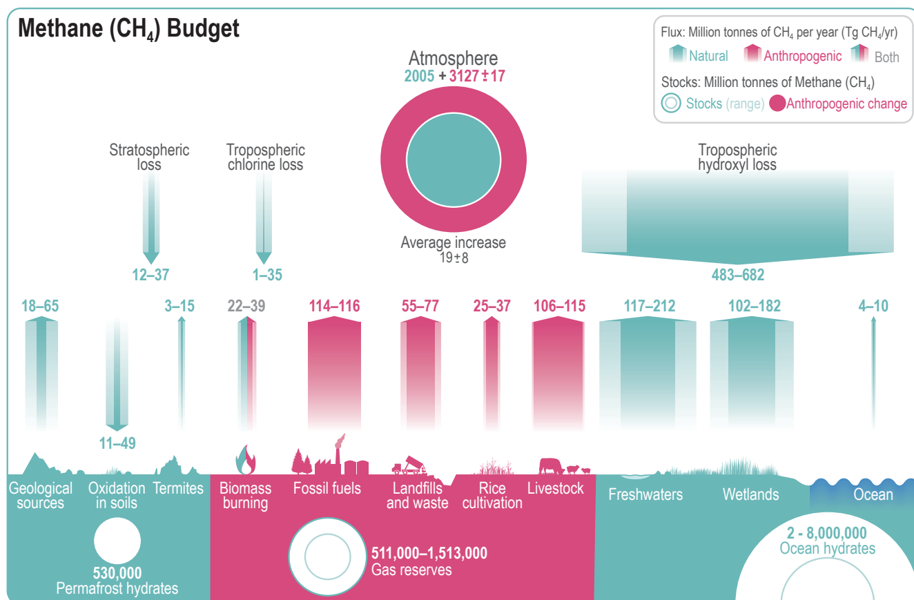
Figure 5.14 | Global methane (CH 4 ) budget (2008–2017). Values and data sources as in Table 5.2 (in Tg CH 4 ). The atmospheric stock is calculated from mean CH 4 concentration, multiplying a factor of 2.75 \pm 0.015 Tg ppb -1 , which accounts for the uncertainties in global mean CH 4 (Chandra et al., 2021). Further details on data sources and processing are available in the chapter data table (Table 5.SM.6).
