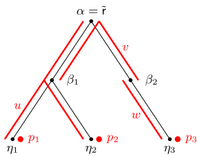
(a) The tree representation (\tilde{T}, \mathcal{M}_{|V(\tilde{G})}) of \tilde{G} where V(\tilde{G}) = \{p_1, p_2, p_3, u, v, w\} and \tilde{P}_r = \emptyset . (b) The instance (H_2, s, \tilde{r}, \text{wt}_2) (thick arcs have infinite weight).
