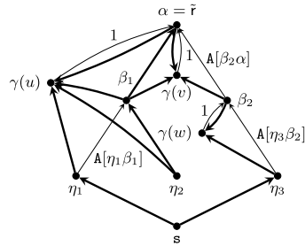
(a) The tree representation (\tilde{T}, \mathcal{M}_{|V(\tilde{G})}) of \tilde{G} where V(\tilde{G}) = \{p_1, p_2, p_3, u, v, w\} and \tilde{P}_r = \emptyset . (b) The instance (H_2, s, \tilde{r}, \text{wt}_2) (thick arcs have infinite weight).
