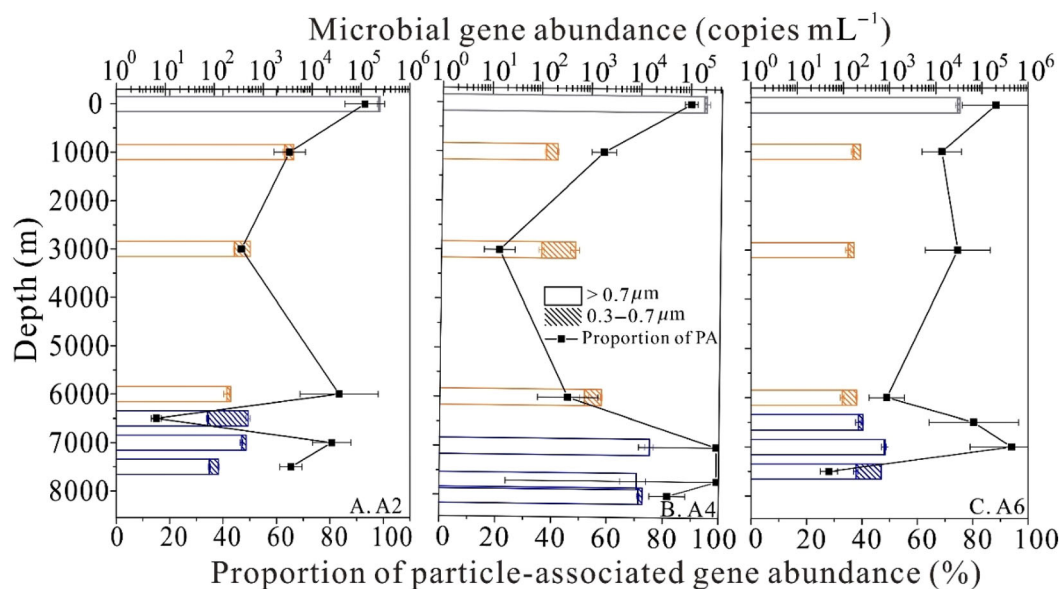
Fig. 4. The log scale of microbial gene abundance on particle-associated (PA, > 0.7 \mu\text{m} , or sum of 0.7\text{--}2.7 \mu\text{m} and > 2.7 \mu\text{m} fractions) and free-living ( 0.3\text{--}0.7 \mu\text{m} ) microbial community (copies \text{mL}^{-1} ) based on 16s rRNA analysis at selected sites of (A) A2, (B) A4, and (C) A6 in the Atacama Trench. Bars of light blue, orange, and dark blue represented epipelagic, dark ocean, and hadopelagic zone, respectively. The black dotted line indicated the % proportion of the particle-associated gene abundance at each site.
