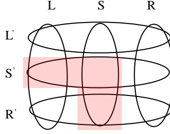
Figure 1: A crossing-diagram for two separation triples (L, S, R) and (L', S', R') . The neighbors of L \cap R' is a subset of (R' \cap S) \cup (S' \setminus R) .
