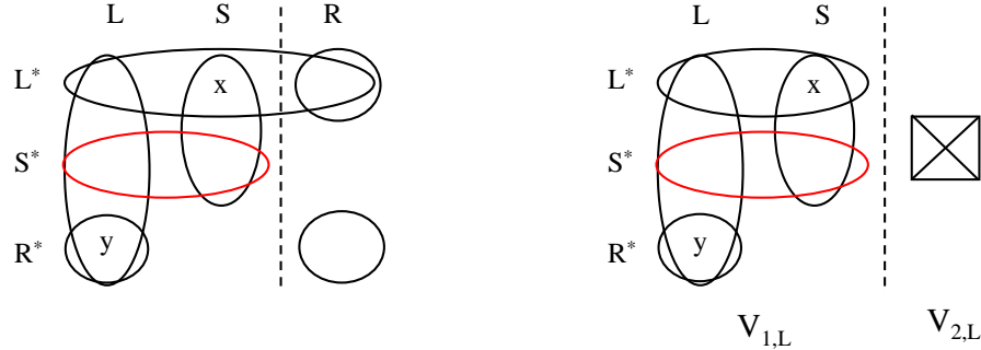
Figure 2: A crossing-diagram for two separation triples (L, S, R) and (L^*, S^*, R^*) before and after transformation from G to H_L .
