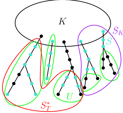
Figure 3: Cases 2a and 2b of Lemma 8.13. The set S is the cyan vertices.
