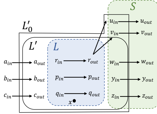
Figure 1: Construction of a separation triple (L, S, R) in G from an edge cut L' in G' . Most edges are omitted. From this example, L'_0 = L' \cup \{u_{in}, v_{in}\} , L = \{r, p, q, x\} , S = \{u, v, w, y, z\} .
