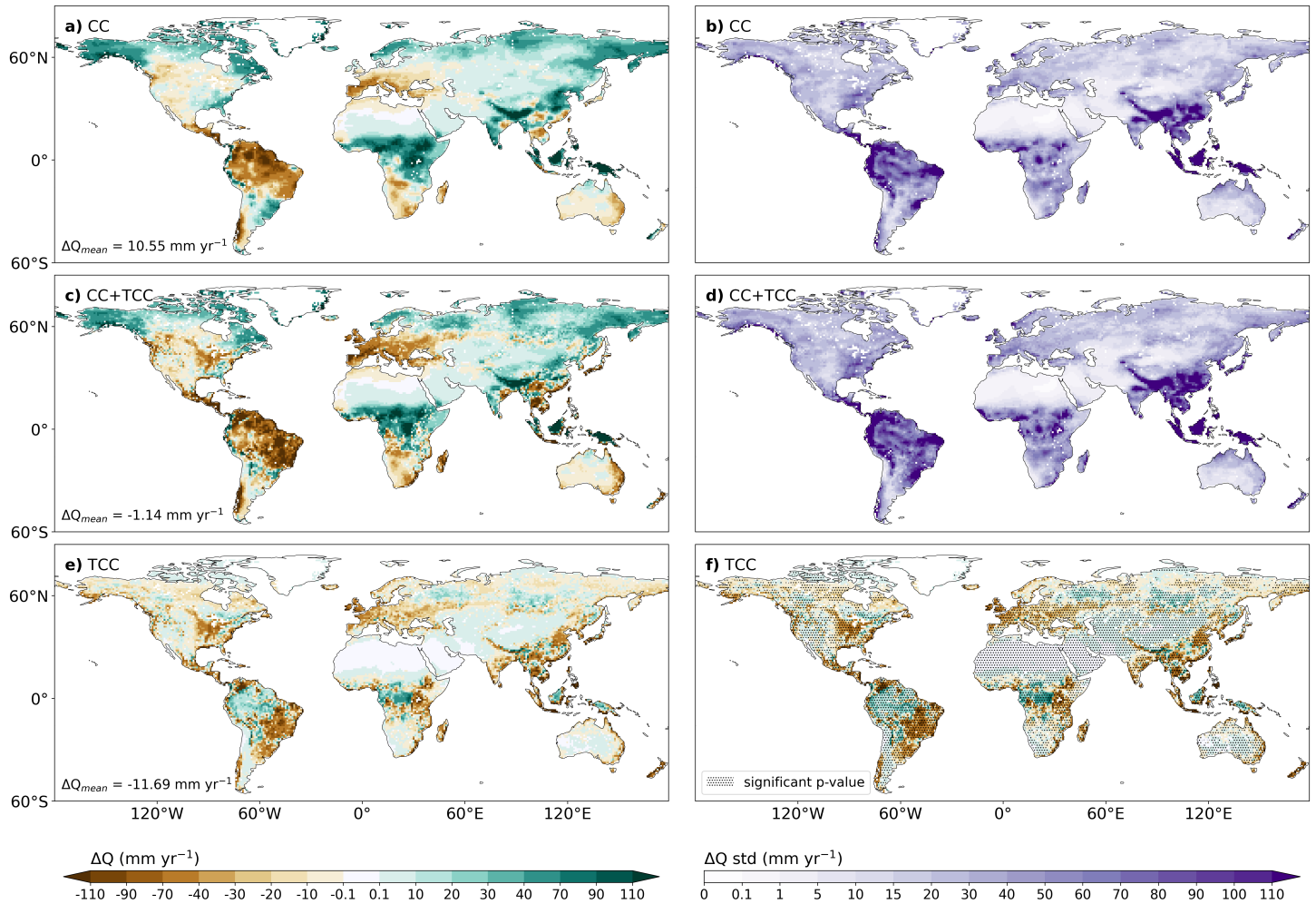
Figure 5. Average runoff change ( \Delta Q : a, c, e, and f) and the corresponding standard deviation (b and d) in a future climate due to the impact of climate change (CC; a and b) and the combined impacts of climate change and tree cover change (CC + TCC; c and d). The hydrological changes in these figures are relative to the present climate. Figures e and f both display the impact of tree cover change (TCC; difference between CC and CC+TCC), whereby figure f illustrates the spatial significance for \Delta Q due to TCC. The spatial significance is obtained by applying a Wilcoxon Signed-Rank Test to every land grid cell and the stippling in the figure indicates which grid cells have a significant p-value ( <0.05 ).
