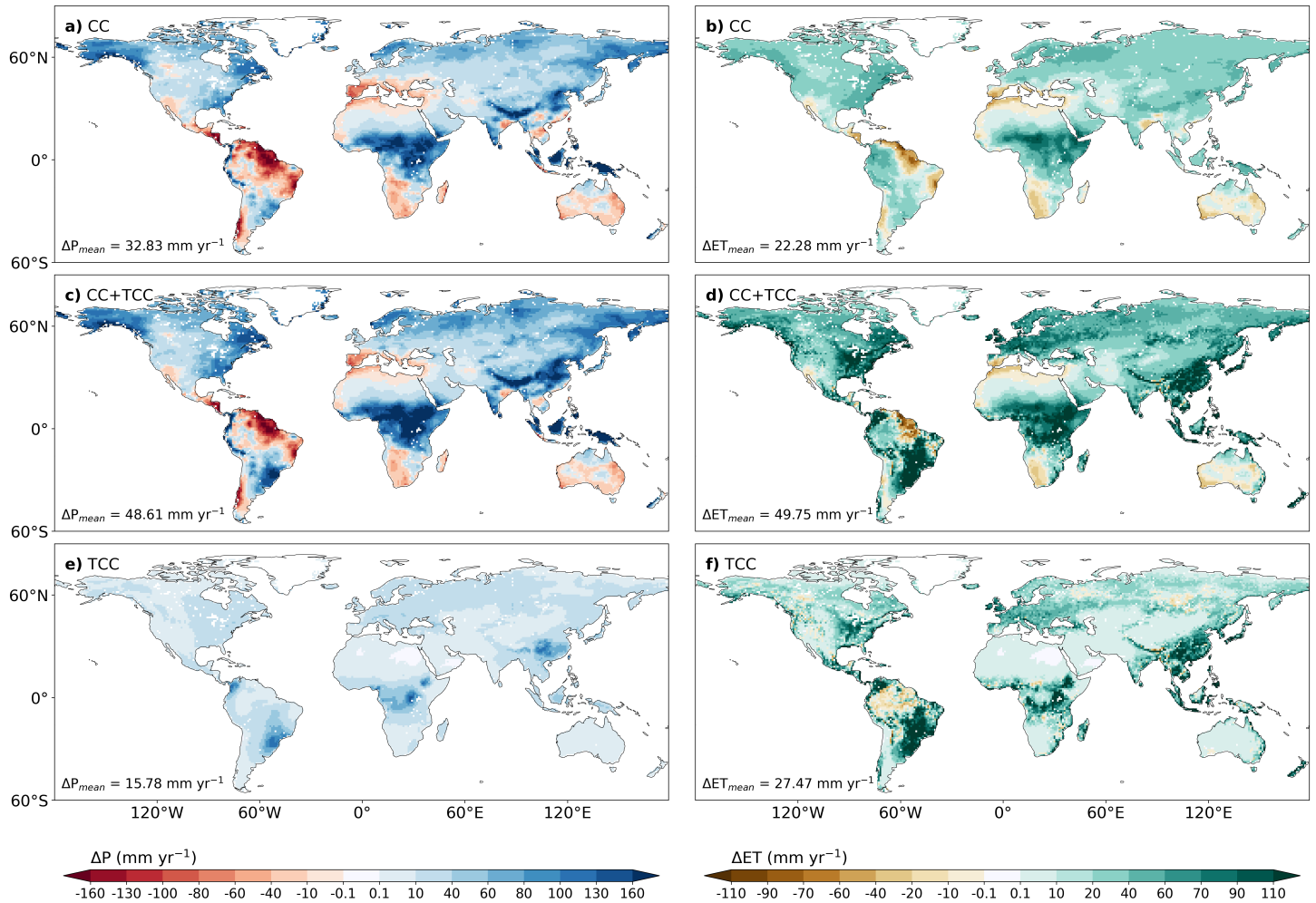
Figure 4. Average precipitation change ( \Delta P ; left) and evapotranspiration change ( \Delta ET ; right) in a future climate due to the impact of climate change (CC; a and b) and the combined impacts of climate change and tree cover change (CC + TCC; c and d). The hydrological changes in these figures are relative to the present climate. Figures e and f only display the impact of tree cover change (TCC; difference between CC and CC+TCC).
