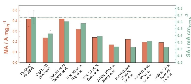
Figure 5. Mass activity (MA) and specific activity (SA) of Pt 27 Co 1 /C via ZIF-8 encapsulation versus direct deposition of the metal nanocluster on carbon (“Co 8 Pt 4 NC/Vulcan®”) evaluated at 0.9 V vs RHE in 0.1 M HClO 4 at a rotation speed of 1600 rpm. MA and SA values of commercial Pt/C Tanaka, E-TEK, and HISPEC Pt/C catalysts are added from the literature to compare the ORR activity of Pt 27 Co 1 /C via ZIF-8 catalyst synthesized in this work with state-of-the-art Pt/C catalysts. Dotted orange and green lines mark the highest mass and specific activity, respectively, achieved among the ORR catalysts presented here.
