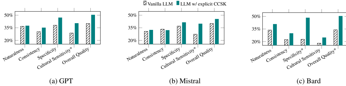
Figure 2: Results of head-to-head comparison for the next utterance generation task via human evaluation. The y-axis represents the percentage of samples preferred by the evaluators (the “Tie” cases are omitted from the plots). The (*) marker indicates results with statistically significant differences ( p < 0.05 in the Wilcoxon T-test).
