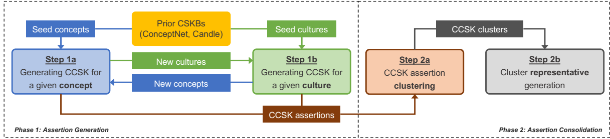
Figure 1: MANGO’s CCSK distillation workflow. Examples for each step can be found in Table 1.
