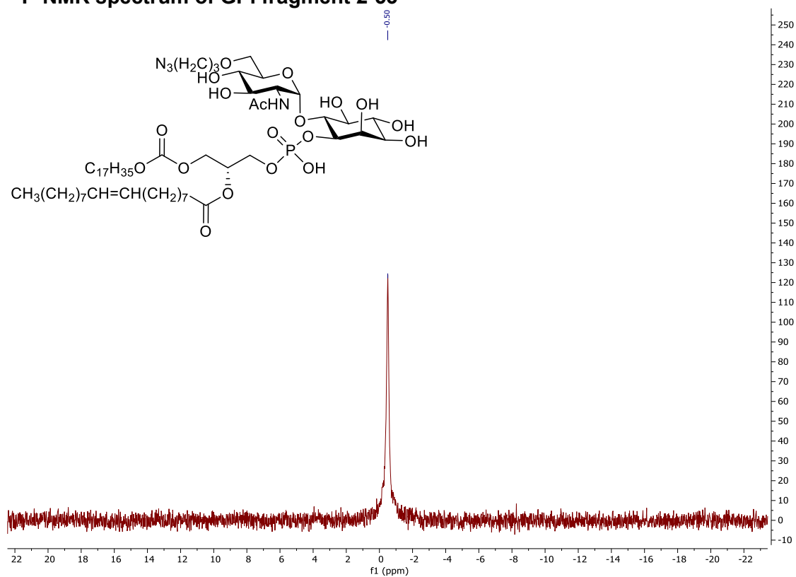
^{31}P -NMR spectrum of GPI fragment 2-53
