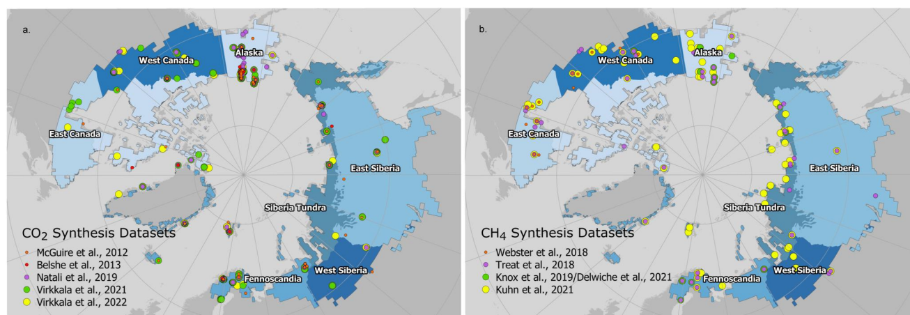
Figure 2. Maps showing the distribution of measurement sites included in existing synthesis products for both (a) CO 2 flux data syntheses (adapted from Virkkala et al., 2022); and (b) CH 4 flux data syntheses including both eddy covariance (FLUXNet; Delwiche et al., 2021; Knox et al., 2019), as well as eddy covariance and chambers covering both growing season, and annual emissions (Kuhn et al., 2021a; Treat et al., 2018a; Webster et al., 2018). The regions used in the analysis are labeled indicated in different shades of blue.
