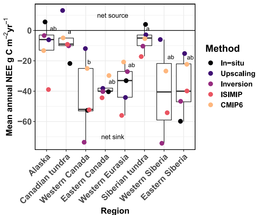
Figure 4. A comparison of regional terrestrial annual NEE over 2002–2014 across the main model and synthesis categories. Regional differences in NEE were statistically significant ( p = 0.0014 ). Each region that shares a mean not statistically different ( p > 0.05 ) from another one based on Tukey’s test shares the same letter.
