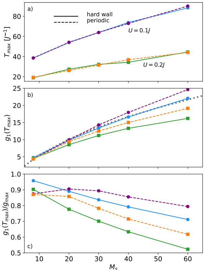
Figure 11. Dynamical quasi-condensation as functions of system size M_s . (a) T_{\max} , (b) g_1(T_{\max}) , and (c) g_1(T_{\max}) relative to the maximum g_{\max} (Eq. 15) for hard-wall boundary conditions (solid), periodic boundary conditions (dashed), U = 0.1J (dots), and U = 0.2J (squares). The gray dotted line in (b) corresponds to a fit to a square root function.
