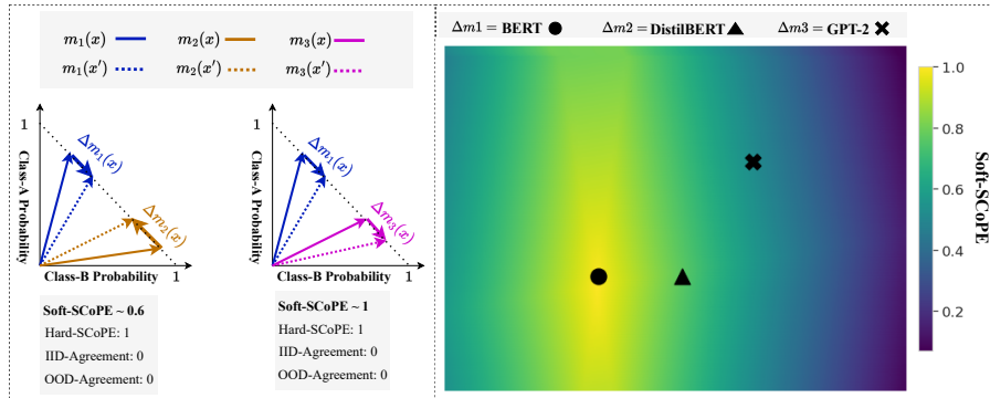
Figure 1: Left : Probability vectors for three models ( m_1 , m_2 , and m_3 ) trained on a binary classification task. For perturbation ( x \rightarrow x' ) defined w.r.t m_1 , both m_2 and m_3 satisfy the Hard-SCoPE criteria. However, the effect of the perturbation is more aligned for m_1 & m_3 (blue and purple) compared to m_1 & m_2 (blue and brown). Right : 2-D Soft-SCoPE surface for a pair of base and perturbed samples, where the reference model BERT is compared with DistilBERT and GPT-2.
