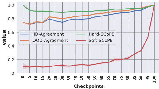
Figure 9: [Reference Model: final-checkpoint i.e. 100% pre-training , Target Model: m_t for t\% pre-training, Linguistic-Capability: Synonym-Invariance ] Comparing different metrics to analyze how intermediate-checkpoints share capabilities on Synonym-Invariance defined w.r.t the final-checkpoint. Even though the initial-checkpoint (0% pre-training) is not much better than a random-baseline, it shares a high-degree of Hard-SCoPE and IID/OOD-Agreements. Whereas Soft-SCoPE grows in a gradual manner over the course of pre-training.
