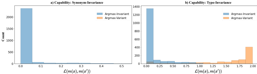
Figure 11: [Reference Model: BERT ] Distribution of \mathcal{L}(m(x), m(x')) for x' \in X' generated along Synonym-Invariance and Typo-Invariance. We note that the distribution is skewed towards lower \mathcal{L}(m(x), m(x')) values and most samples generated are at least invariant in predictions (argmax-invariant).
