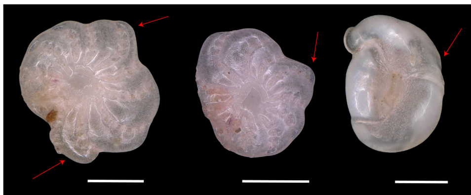
Fig. 11. Side views of malformed tests from sample TR18-107. The arrows point to malformation features such as dwarf chambers or an accessory chamber. Scale bar = 200 \mu\text{m} .
