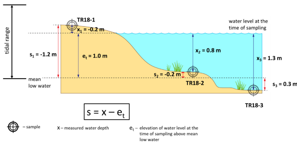
Fig. 2. Calculation of standardised water depth ( s ) from measured water depth ( x ). Standardised water depths are given as positive values of distances between the mean low-water level and the sampling point if it lays below low-water level and as negative values if above the low-water level.
