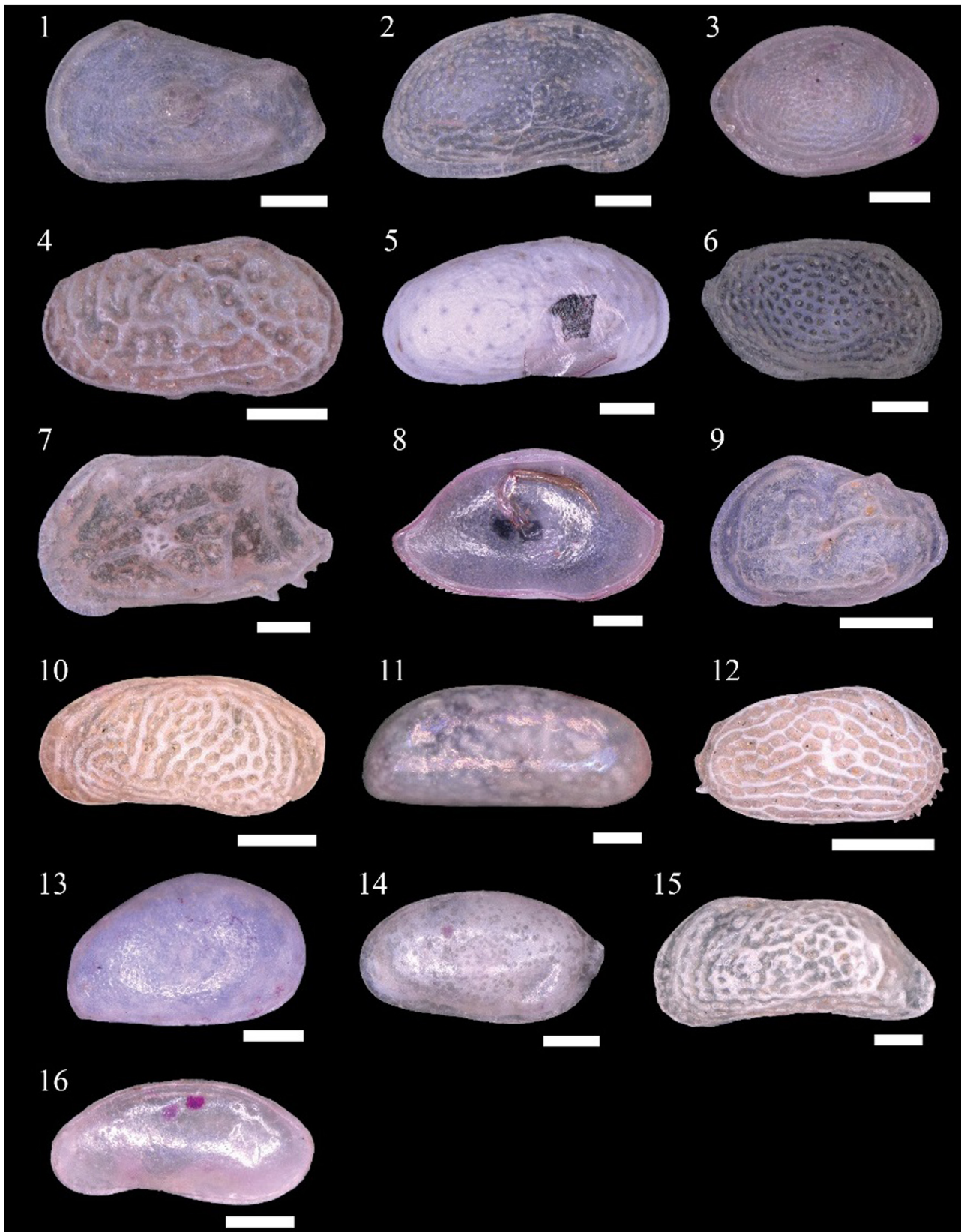
Fig. 8. Ostracod taxa of uMlalazi Estuary. All pictures are giving external views if not stated otherwise; all of them are light microscope photos. Scale bar length = 100 \mu m. (1) Ambostracon sp., LV, sample TR18–83; (2) Aurila kliei (Hartmann, 1974), RV, TR18–83; (3) Australoloxoconcha favornamentata (Hartmann, 1974), RV, TR18–90; (4) Callistocythere cf. eulitoralis (Hartmann, 1974), RV, TR18–83; (5) Cytheromorpha ?milleri (Dingle and Honigstein, 1994), RV, TR18–84; (6) Loxococoncha sp., RV, TR18–83; (7) Mutilus bensonmaddocksorum (Hartmann, 1974), LV, TR18–83; (8) Neonesidea sp., LV, internal view, TR18–83; (9) Sulcostocythere knysnaensis (Benson and Maddocks, 1964), LV, juvenile, TR18–84; (10) Tanella africana (Hartmann, 1974), RV, TR18–89; (11) Argilloecia sp., RV, TR18–83; (12) Ruggieria sp., RV, juvenile, TR18–83; (13) Cyprideis sp., RV; juvenile, TR18–84 (14) Paradoxostoma griseum (Klie, 1940), LV, TR18–83; (15); Perissocytheridea estuaria (Benson and Maddocks, 1964), LV, TR18–85; (16) Sclerochilus sp., RV, TR18–83;
