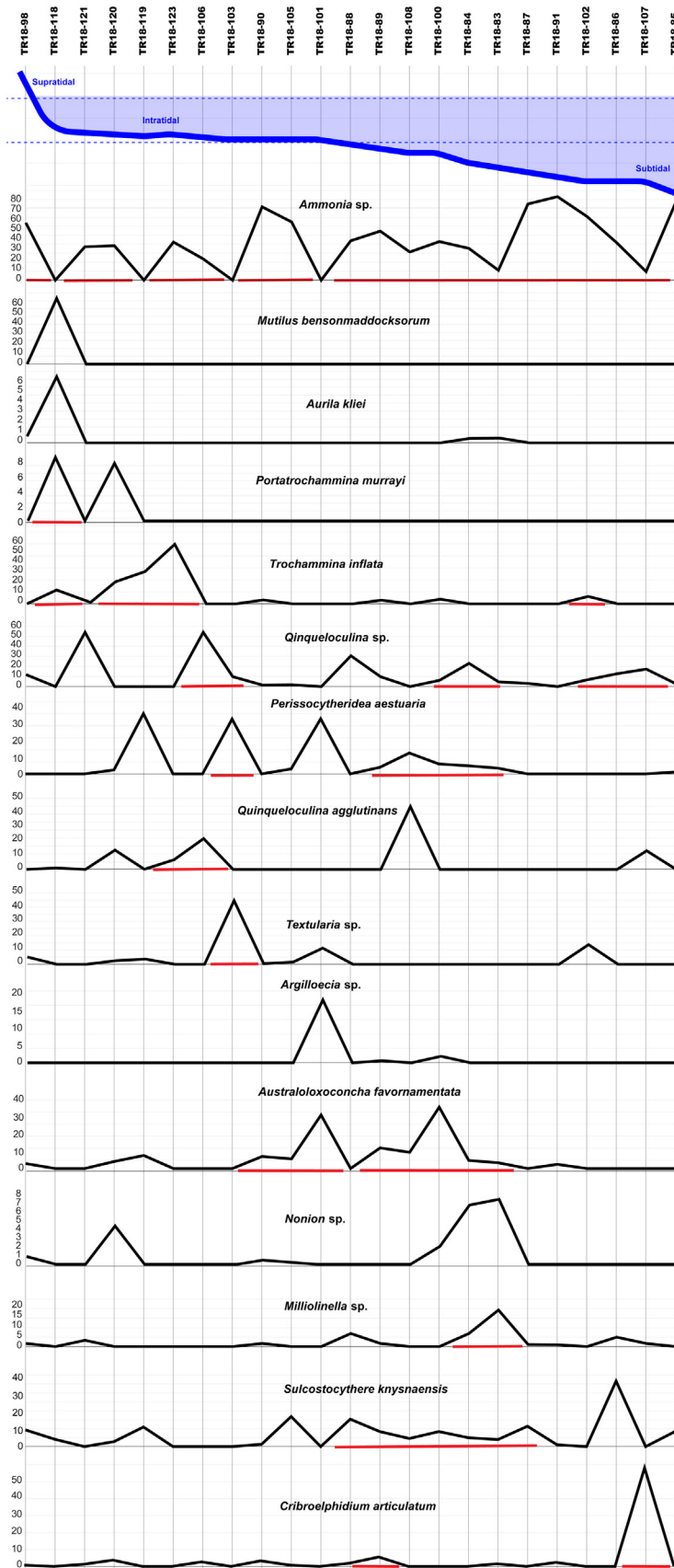
Fig. 13. Elevation-bound distribution patterns of Foraminifera and Ostracoda. Red lines indicate occurrences of living individuals. Y axis shows relative abundances.
