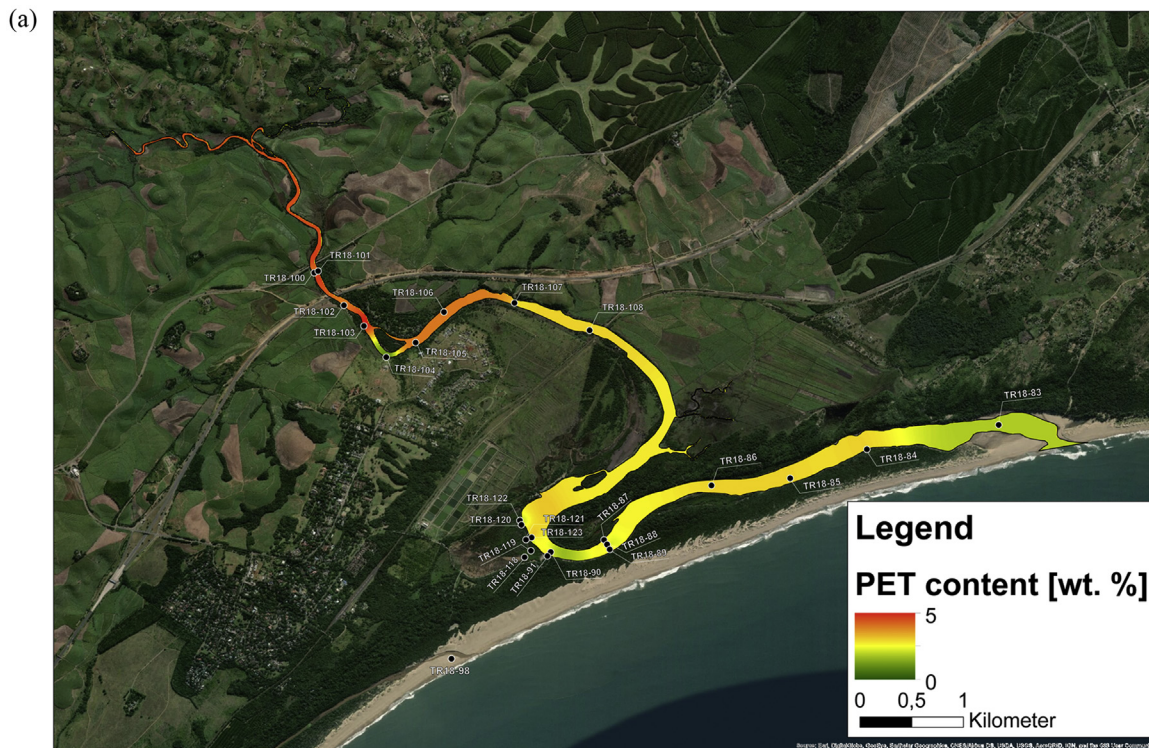
Fig. 7. Distribution of a) PET and b) of LDPE within the sediment samples.
