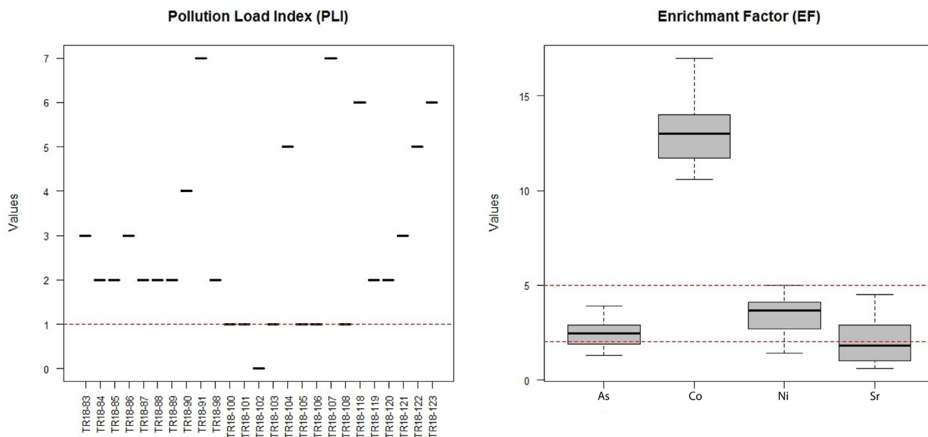
Fig. 4. Pollution Load Index (left) and Enrichment Factor (right) based on EFs of As, Co, Ni and Sr. The tick line inside the boxes is the median of the dataset. The red dashed lines are the thresholds (see Tables 2, 3). The shown heavy metals displayed the highest values.
