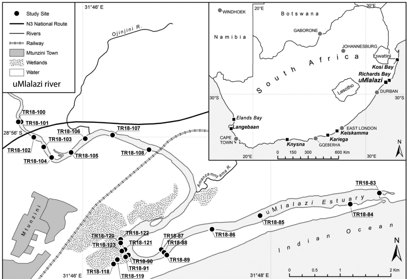
Fig. 1. The location of uMlalazi river in South Africa with the sampling stations in 2018, except TR18–98 which was collected near a small creek that ran from the river at the beach line (see Fig. 12).
