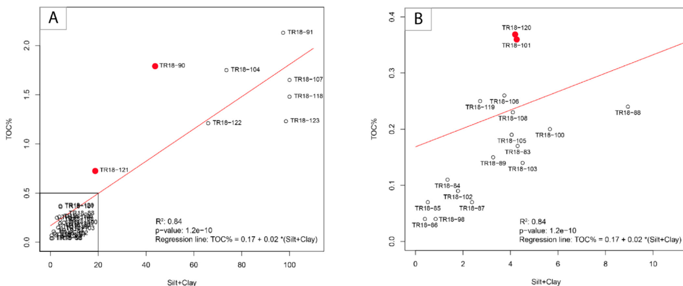
Fig. 5. a) fine grain material silt+clay against the percentage of TOC. b) zoomed in distribution. Samples marked in red are enriched in organic carbon.
