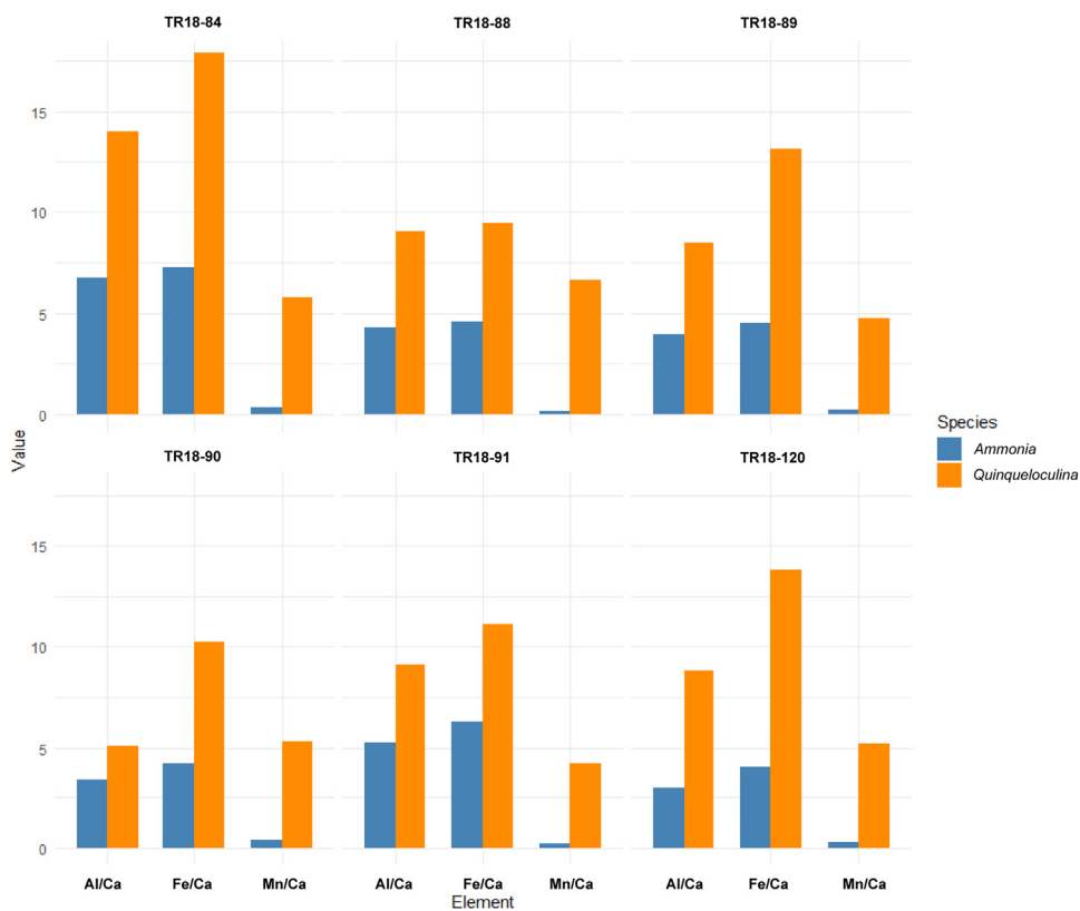
Fig. 6. Al/Ca, Fe/Ca and Mn/Ca ratios of Quinqueloculina sp. and Ammonia sp.
