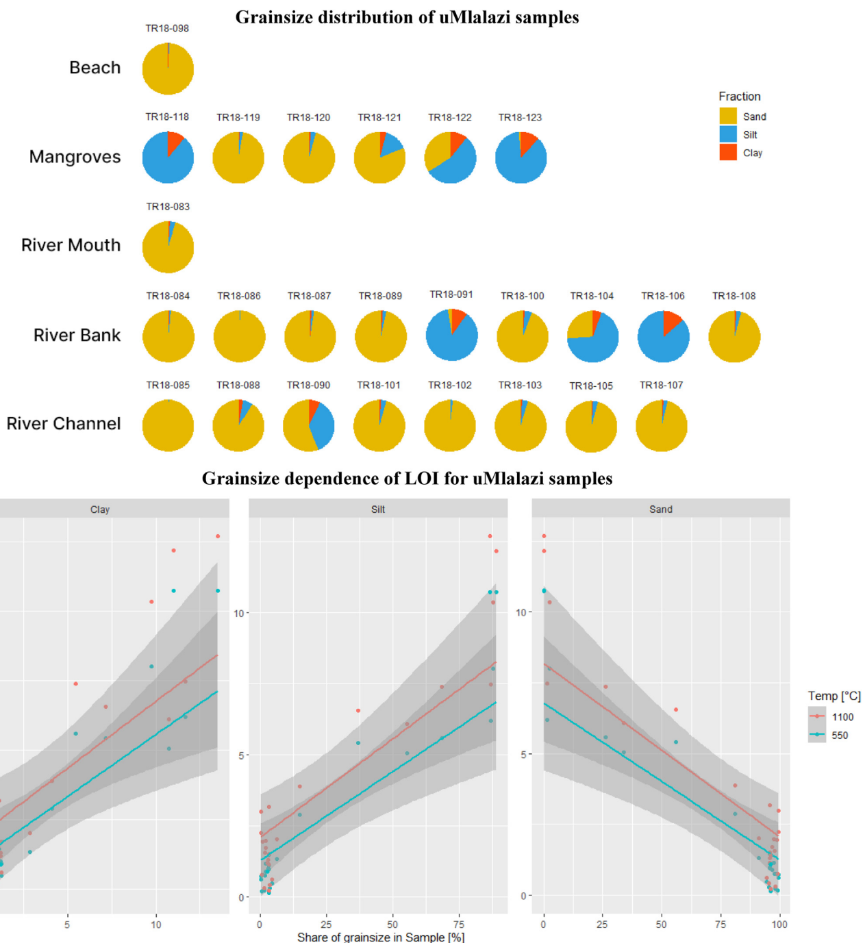
Fig. 3. Grainsize distribution and grainsize-dependence of LOI of uMlalazi samples.
