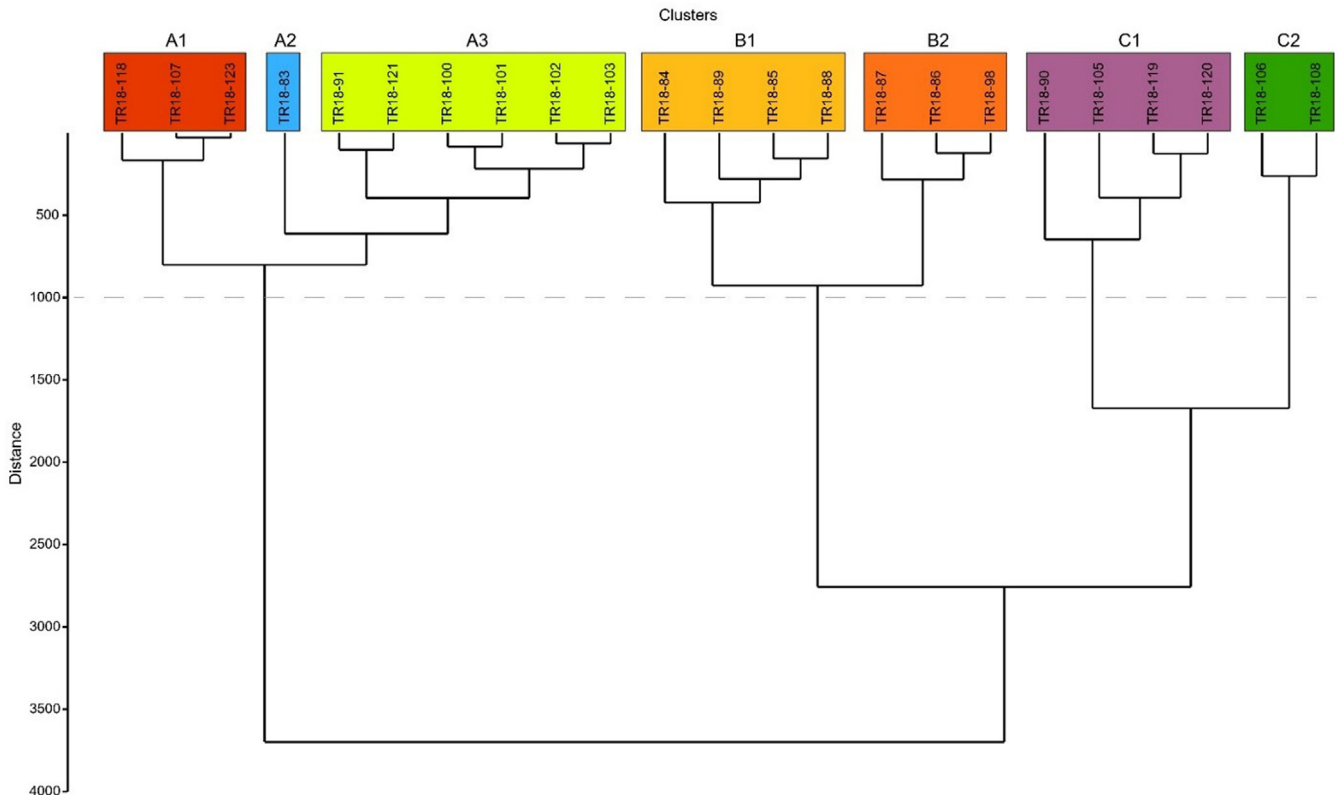
Fig. 10. The dendrogram of a cluster analysis of microfossil distribution.
