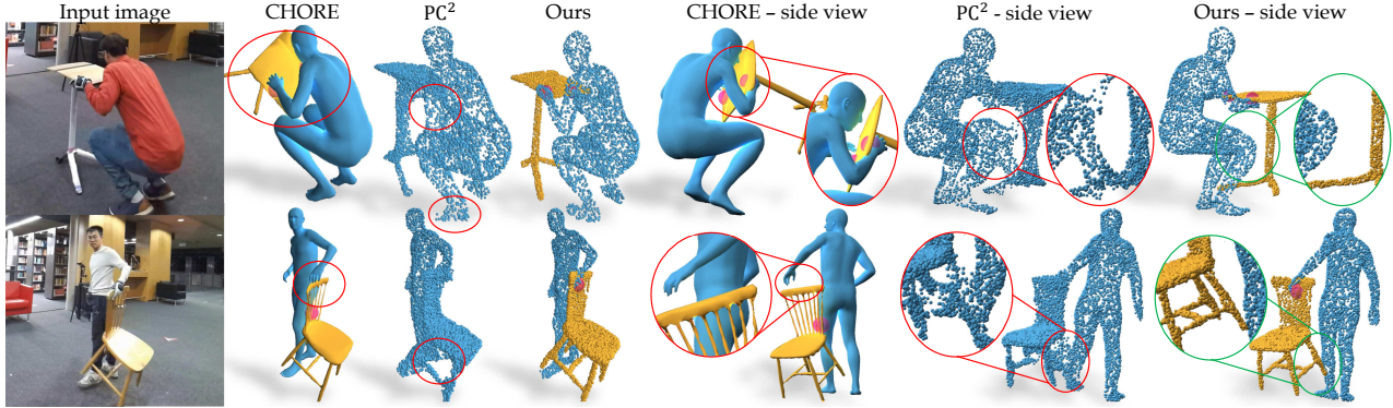
Figure 4. Comparing reconstruction results on BEHAVE[7] dataset. CHORE[87] relies on object mesh templates and the prediction is inaccurate for challenging poses. PC 2 [56] does not rely on templates but its predicted point clouds are noisy (red circles) and it cannot predict contacts. Ours can reason about human object interaction, and predicts high-fidelity human and object shapes without templates.
