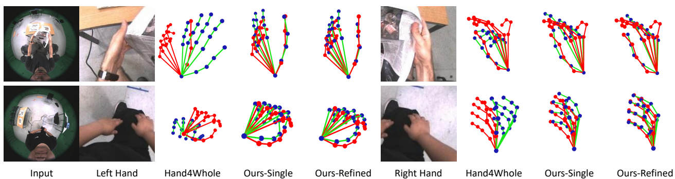
Figure 10. Qualitative comparison on hand pose estimation results. Our single-view and refined hand poses are more accurate than the poses from Hand4Whole [32] method. The red skeleton is the ground truth while the green skeleton is the predicted pose.
