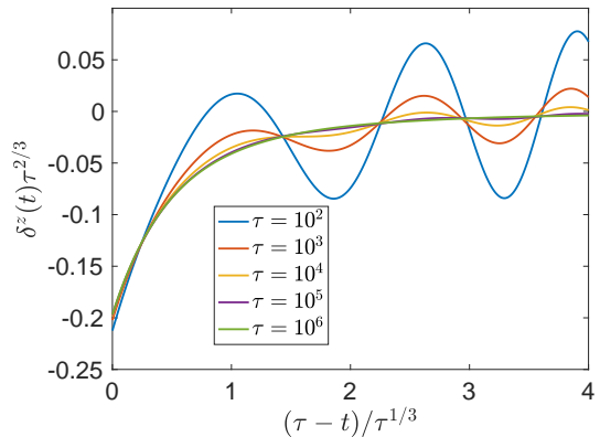
FIG. 2. Temporal data collapse of \delta^z(t) close to the CP for various ramp rates after a ramp from the FM ( g_0 = 0 ). The data is obtained from the numerical solution of Eq. (4). Deviations from zero start to appear at times \sim \tau^{1/3} before reaching the CP. Similar data collapse characterizes the other spin components.
