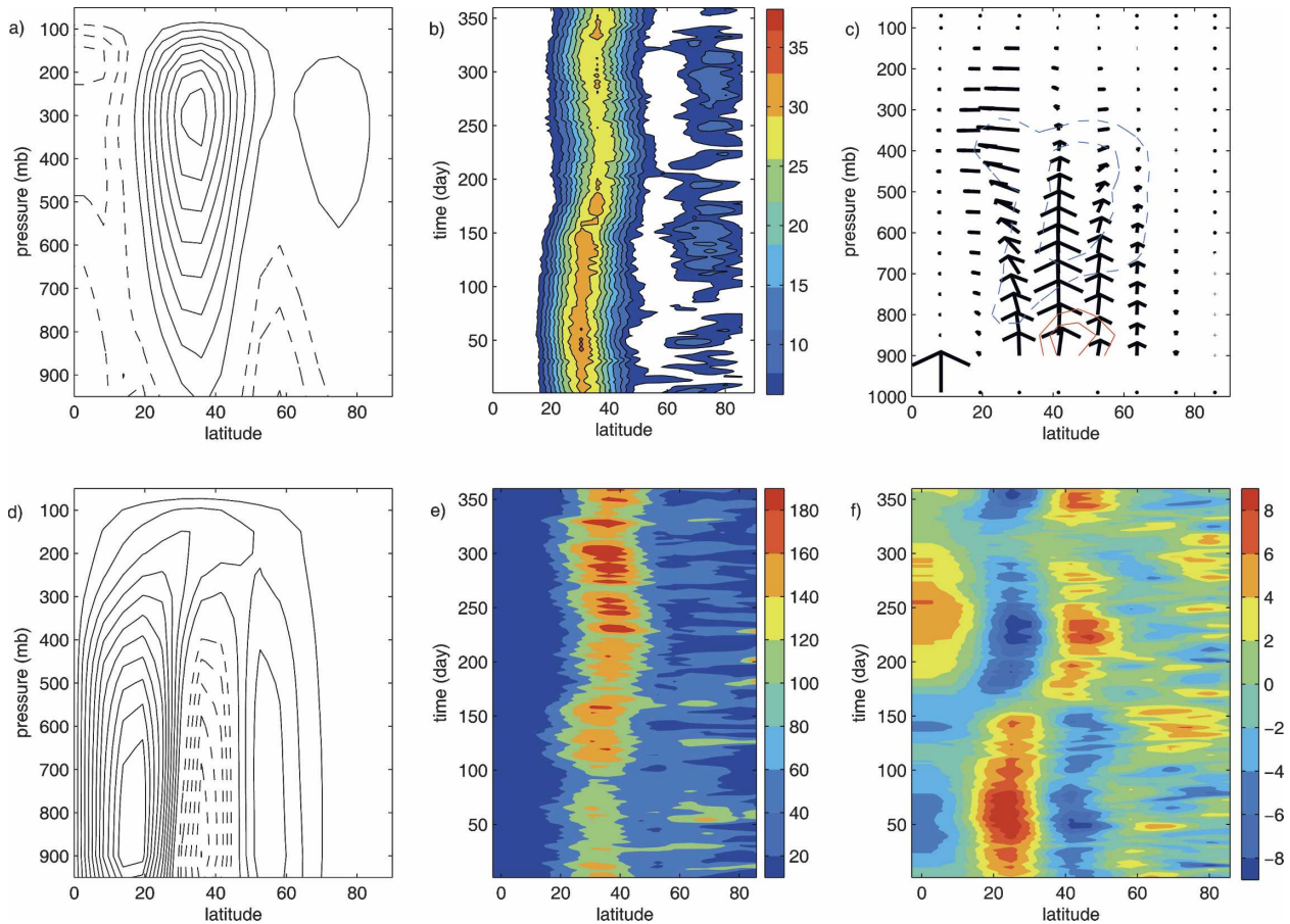
FIG. 5. The C-1b setup: (a) time-averaged (360 days) zonal mean zonal wind, (b) time evolution (Hovmoeller diagram) of the zonal mean zonal wind at 400 mb, (c) E-P flux (arrows) and the flux divergence field, (d) mass streamfunction, (e) zonal mean of the eddy kinetic energy at 500 mb, and (f) time evolution (Hovmoeller diagram) of the zonal mean zonal wind anomaly at 500 mb. Units and contour intervals are the same as in Fig. 4.
