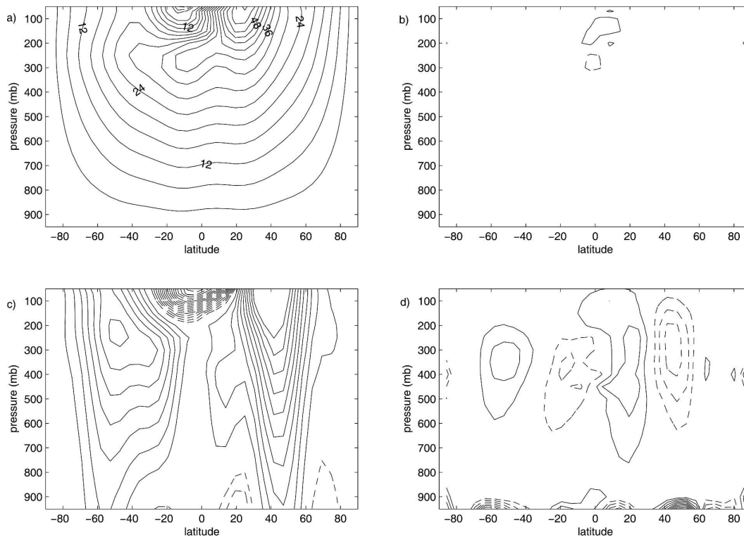
FIG. A2. Solutions for the C-1c setup: averaged zonal mean zonal and meridional wind (a), (b) with no eddies and (c), (d) with eddies. Units and contour intervals are the same as in Fig. 8.
