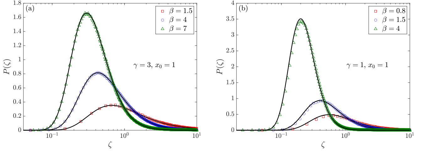
FIG. 4. PDF of the scaled variable \mathcal{Z}/Z_D , with \mathcal{Z} representing the functionals (a) \mathcal{Z} = \int_0^T x(t)dt and (b) \mathcal{Z} = \int_0^T [x(t)]^{-1}dt for trajectories in the positive real axis starting from x_0 = 1 and evolved up to the first-passage time to the origin. The diffusion coefficient is set to one. The solid black curves are the theoretical predictions given by Eq. (115), the symbols represent the numerical distributions obtained from simulations. For both values of \gamma we considered different values of \beta : (a) in the case \gamma = 3 we choose \beta = 1.5 (red squares), \beta = 4 (blue circles) and \beta = 7 (green triangles), (b) in the case \gamma = 1 we take \beta = 0.8 (red squares), \beta = 1.5 (blue circles) and \beta = 4 (green triangles). The number of simulations depends on \beta : for \beta = 0.8 and \beta = 1.5 it is 3 \cdot 10^5 , for \beta = 4 and \beta = 7 it is 3 \cdot 10^6 . All the trajectories are evolved with small time step \Delta t = 10^{-5} .
