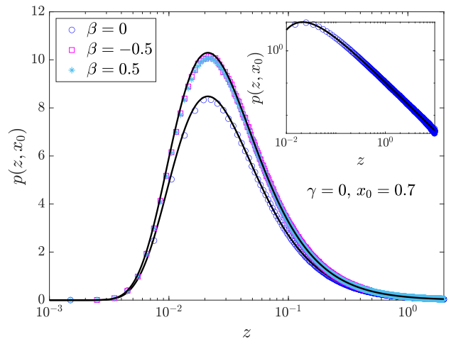
FIG. 3. PDF of the functional \mathcal{Z} = \int_0^T [x(t)]^{-2} dt for trajectories in \Omega = (0, 1) . The starting point is x_0 = 0.7 and the diffusion coefficient is set to one. The solid black curves are the theoretical predictions given by Eq. (98), the symbols represent the numerical distributions obtained from simulations. We have considered \beta = -0.5 (magenta squares), \beta = 0 (blue circles) and \beta = 0.5 (turquoise asterisks), with good agreement in all cases. Note that data corresponding to the same |\beta| overlap, confirming the symmetry in \beta of the PDF. In the inset, a plot in logarithmic scale of the case \beta = 0 , which shows that the simulations also capture the heavy tail of the distribution. The number of simulations is 10^8 for \beta = 0.5 and 10^7 in the other cases. The trajectories are evolved up to the first-passage time with small time step \Delta t = 10^{-5} .
