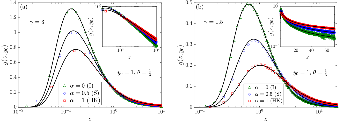
FIG. 5. PDF of (a) \mathcal{Z} = \int_0^T y(t) dt and (b) \mathcal{Z} = \int_0^T [y(t)]^{-1/2} dt for trajectories in the positive real axis generated by Eq. (117) and evolved up to the first-passage time to the origin. The starting point is y_0 = 1 and the space-dependent diffusion coefficient is D(x) = x^{2/3} . The solid black curves are the theoretical predictions given by Eq. (128), the symbols represent the numerical distributions obtained from simulations. For both values of \gamma we considered three different interpretations, corresponding to Itô ( \alpha = 0 , green triangles), Stratonovich ( \alpha = \frac{1}{2} , blue circles) and Hänggi-Klimontovich ( \alpha = 1 , red squares). The insets, which are presented in log-log scale in (a) and semilog scale in (b), display the heavy-tails of the distributions. All datasets are obtained by evaluating \mathcal{Z} over 10^6 trajectories, with small time step \Delta t = 10^{-4} . The integration scheme used to integrate Eq. (117) is the Itô scheme, and the desired interpretation is obtained by adding the appropriate drift \mu_\alpha(x) = \alpha D'(x) .
