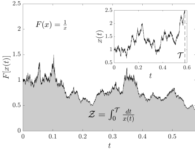
FIG. 1. Example of first-passage functional \mathcal{Z} = \int_0^{\mathcal{T}} F[x(t)]dt for Brownian motion in a potential V(x) = V_0 \ln(x) diffusing in \Omega = (\frac{1}{2}, \frac{5}{2}) . Here F(x) = 1/x and \mathcal{Z} thus corresponds to the area under the graph of 1/x(t) , where x(t) is the stochastic trajectory displayed in the inset. The trajectory starts from x_0 = 1 and the motion is evolved up to the first-exit time from \Omega . The diffusion constant is equal to one and V_0 = 0.5 .
