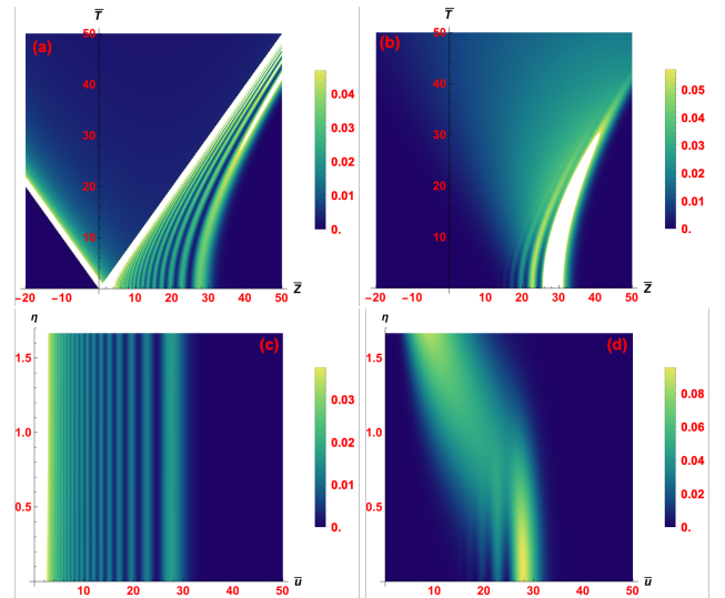
Figure 1. Spacetime profile of the electron density for the free electron modulated wavepacket of Eq. (13): (a,b) in the Lab-frame; (c,d) in the accelerated frame (i.e., in Rindler coordinates); (a,c) \alpha = 30 and \bar{a} = 0.005 ; (b,d) \alpha = 30 and \bar{a} = 2 . Note that the Rindler coordinates only cover the region outside the light-cone to the right.
