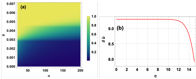
Figure 2. (a) The asymmetry ratio \mathcal{A} = (|\bar{\psi}_R|^2 - |\psi|^2)/(|\bar{\psi}_R|^2 + |\psi|^2) vs the wavepacket chirping parameter \alpha and the size parameter \bar{a} for T = 1 fs; (b) The wavepacket size \delta\bar{u} vs \eta for \alpha = 40 and \bar{a} = 10^{-6} .
