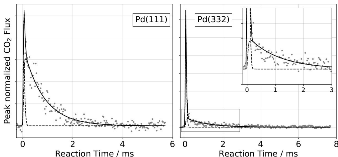
Figure 1: Observation of two temporally resolved CO 2 formation channels in formic acid decomposition on Pd. Typical peak normalized kinetic traces of CO 2 on Pd(111) (left) and Pd(332) (right) at 403 K using HCOOH. The VRK data are fit according to Eq. 2 (Pd(111): k_1 > 80\,000\text{ s}^{-1} and k_2 = 1200\text{ s}^{-1} , Pd(332): k_1 > 80\,000\text{ s}^{-1} and k_2 = 900\text{ s}^{-1} ). The inset in the right panel shows an enlarged view of the slow component which decays over several milliseconds at this temperature whereas the fast component is on the timescale of the incident molecular beam (dashed line).
