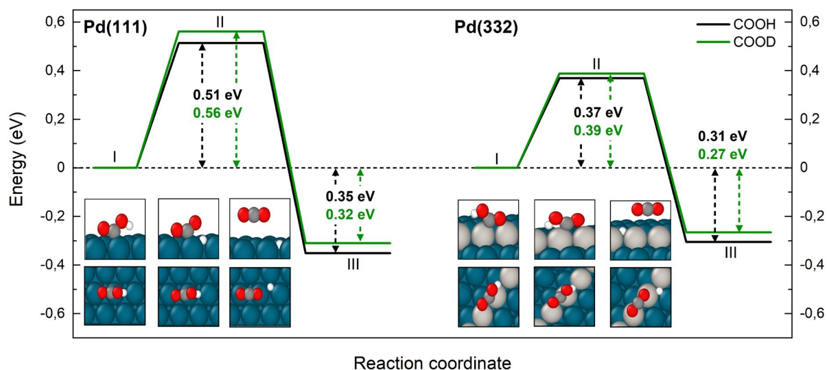
Figure 7: Reaction pathway for CO 2 formation from two isotopologues of carboxyl C*OOH (black) and from C*OOD (green) on Pd(111) and Pd(332) obtained from NEB calculations using PBE-TS functional. On the scheme the initial (I), transition (II) and final state (III) are shown. Atom representation is the same as in Figure 4. The energy values include ZPE correction.
