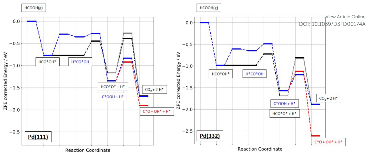
Figure 9: Zero-point energy corrected energy diagram of formic acid decomposition on Pd(111) and Pd(332). The black lines show the bidentate formate pathway, blue the carboxyl to CO 2 pathway and red the carboxyl to CO pathway. The grey line shows the alternative pathway for bidentate formate dissociation as shown in Figure 6b).
