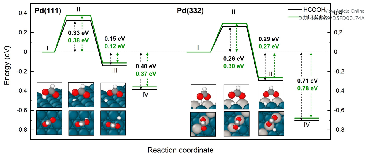
Figure 4: Reaction pathways to form bidentate formate from HCOOH (black) and from HCOOD (green) on Pd(111) and Pd(332) obtained from NEB calculations using PBE-TS functional. Initial (I), transition (II) and final states (III) are shown. Energy level IV correspond to final state (III) without interaction between products. O-atoms are shown in red, C-atoms in dark grey, H-atoms in white, and Pd-atoms in cyan. The Pd-atoms on the steps are distinguished by a light grey color. The energy values include ZPE correction.
