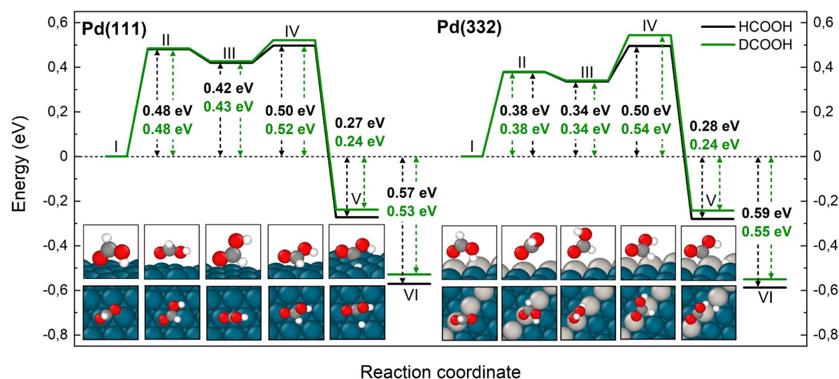
Figure 5: Reaction pathway for carboxyl formation from HCOOH (black) and from DCOOH (green) on Pd(111) and Pd(332) obtained from NEB calculations using PBE-TS functional. On the scheme the initial state (I), the first transition state (II), the intermediate state (III), the second transition state (IV) and the final state (V) are shown. Energy level VI correspond to final state V without interaction between products. Atom representation is the same as in Figure 4. The energy values include ZPE correction.
