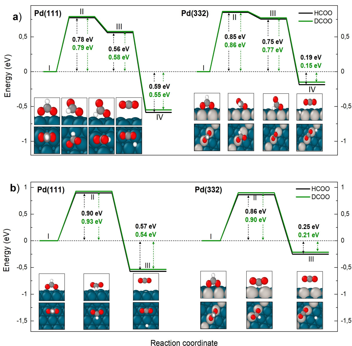
Figure 6: Reaction pathway for carbon dioxide formation from two isotopologues of bidentate formate (HCO*O*) (black) and from DCO*O* (green) on Pd(111) and Pd(332). Panel a) shows the sequential
