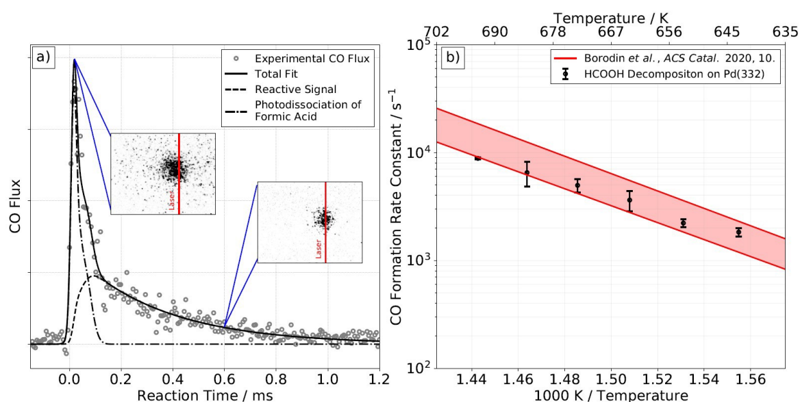
Figure 2: CO formation from formic acid decomposition on Pd. Experimental kinetic trace of CO on Pd(332) at 663 K from HCOOH (left panel, a)) and corresponding Arrhenius plot of the rate constant
