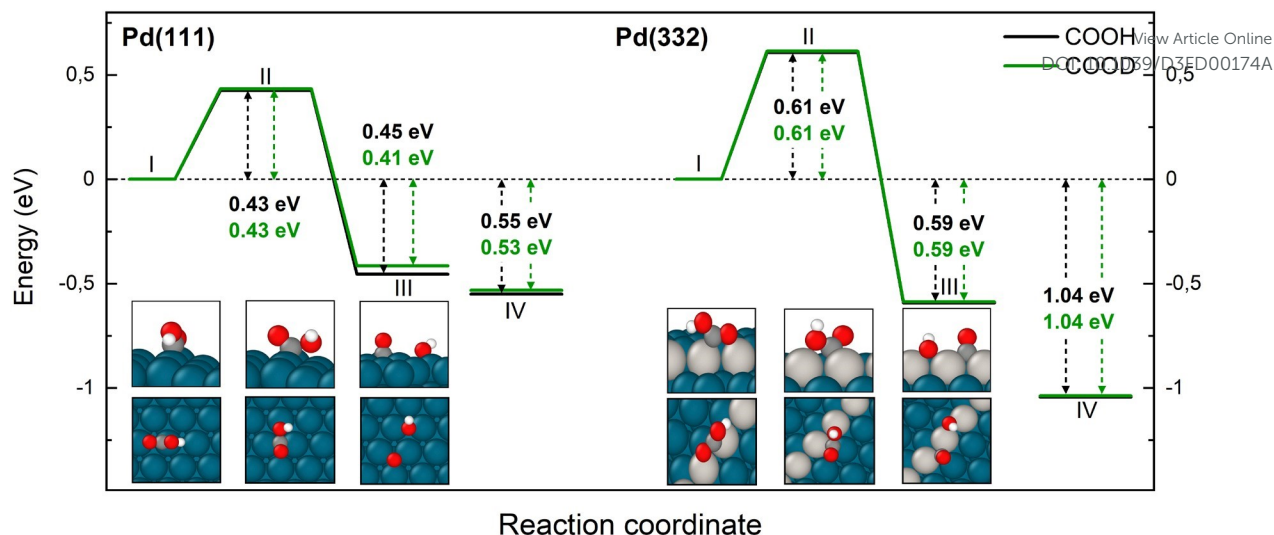
Figure 8: Reaction pathway for CO formation from two isotopologues of carboxyl C*OOH (black) and from C*OOD (green) on Pd(111) and Pd(332) obtained from NEB calculations using PBE-TS functional. In the scheme the initial (I), transition (II) and final state (III) are shown. Energy level IV correspond to final state III without interaction between products. Atom representation is the same as in Figure 4.
