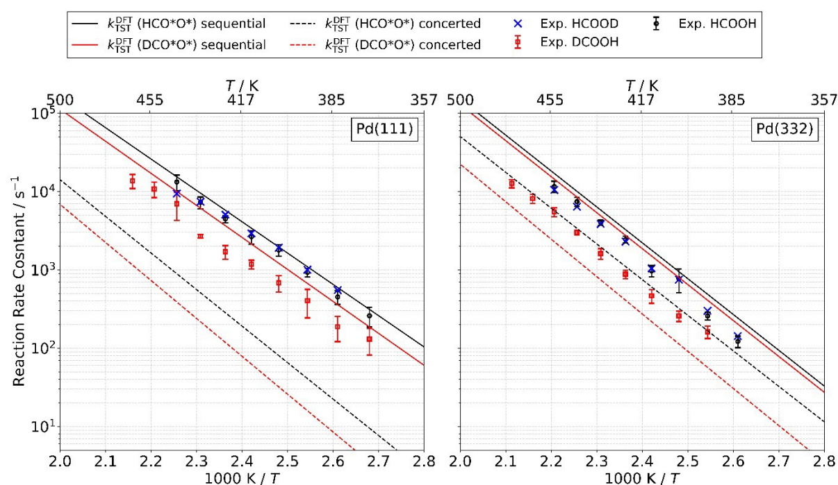
Figure 10: Rate constants for the bidentate formate decomposition to CO 2 (slow channel) from HCOOH (black circles), HCOOD (blue crosses) and DCOOH (red squares) on Pd(111) (left) and Pd(332) (right). Error bars indicate 1 \sigma uncertainty. Within the resolution of our experiment the extracted rate constant for HCOOH and HCOOD are equal. Solid (dashed) lines are predicted rate constants from theory for the sequential (concerted) pathway. See text.
