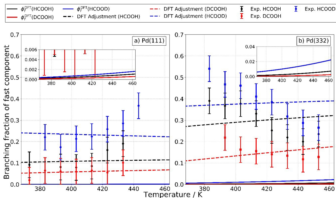
Figure 11: Experimental isotopologue specific branching fractions of the fast component on Pd for different facets and surface temperatures as well as the DFT predicted contribution of the carboxyl intermediate to the total CO 2 formation rate. Panel a) and b) show the experimental branching fractions on Pd(111) and on Pd(332) for HCOOH (black), HCOOD (blue) and DCOOH (red). The error bars indicate a 2 \sigma error interval. The solid lines show the DFT predicted contribution of the carboxyl intermediate to the total CO 2 formation rate. The dashed lines show the predicted results when the DFT based barriers for carboxyl and CO formation on Pd(111) are adjusted by -0.14 and 0.10 eV, respectively and where they are adjusted on Pd(332) by -0.20 eV -0.25 eV, respectively. The branching fraction is in general larger on Pd(332) compared to Pd(111) but have the same trend with isotopologues on both surfaces (DCOOH < HCOOH < HCOOD).
