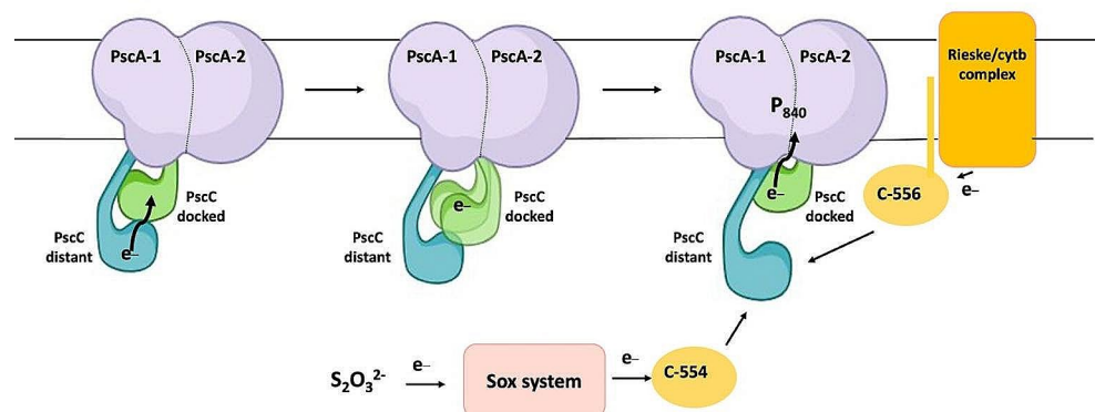
Fig. 6 Model of the electron flow from thiosulfate oxidation via c -554 and from the menaquinol/cytochrome c oxidoreductase via c -556 to the P_{840} special pair
