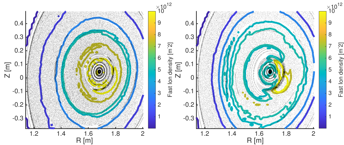
Figure 5: Poincaré traces (black) and fast ion density contours including perturbations using the normal (left) and an increased (right) magnitude.
