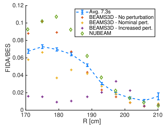
Figure 6: Radial FIDA/BES profiles for the locked mode.
