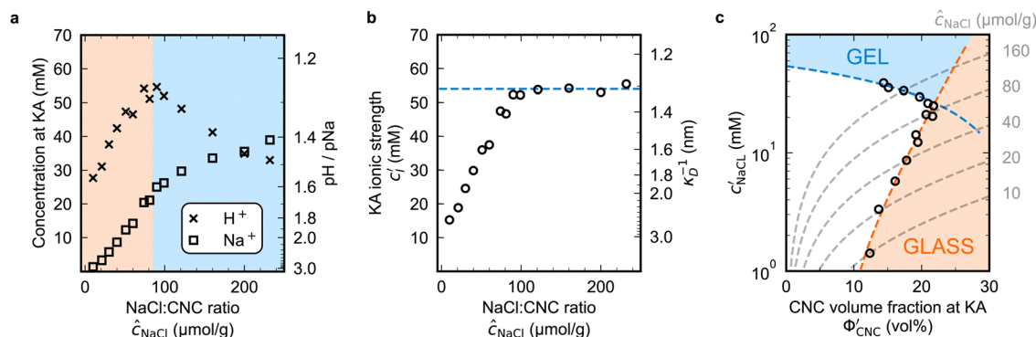
Fig. 5 Ionic composition for H-CNCs with increasing \hat{c}_{\text{NaCl}} : (a) c'_H (crosses) and c'_{\text{Na}} (open squares). Secondary axis shows concentrations expressed as pH/pNa. (b) Ionic strength at KA, c'_I . Secondary y-axis shows the corresponding Debye length \kappa_D^{-1} . Blue dashed line corresponds to an ionic strength of 54 mM and \kappa_D^{-1} \approx 1.3 \text{ nm} . (c) The onset of KA in the (\Phi'_{\text{CNC}}, c'_{\text{NaCl}}) parameter space. Blue dashed line as in (b). Orange dashed line is a guide to the eye. Grey dashed lines indicate the trajectories taken upon drying for CNC suspensions with various \hat{c}_{\text{NaCl}} values.
