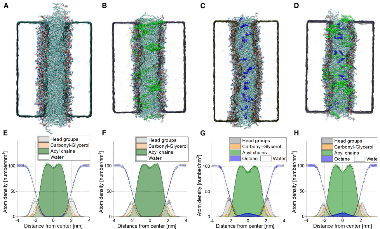
FIGURE 4 MD simulations of symmetric POPC and POPC:POPA 80:20 planar membranes without ( A and B ) and with \sim 13 mol % octane ( C and D ). ( A – D ) Snapshots of the bilayers: The POPC molecules are shown colored according to atom type, POPA is shown in green and octane in blue. ( E – H ) Density profiles of the investigated symmetric systems. To see this figure in color, go online.
