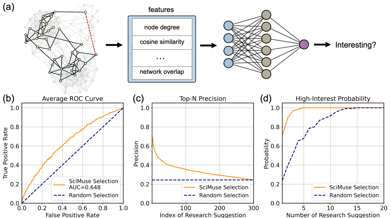
FIG. 4. Learning Scientific Interest. (a), We use the evaluations from research group leaders to train a neural network. This model predicts whether research suggestions are assigned an interest level of 4 or 5 (on a 5-point scale) or below 4, thereby setting up a binary classification task. The input to the neural network consists of 25 features from the knowledge graph of a concept pair, and its output is a single number indicating whether the concept pair is highly interesting (i.e., interest level is \geq 4 ) or not. Given the small size of our training dataset, which comprises a total of 2,996 evaluated research suggestions generated through our knowledge graph, we employ Monte Carlo cross-validation to determine the accuracy of our learning process. (b), The ROC curve indicates that we can correctly predict a randomly chosen highly interesting concept pair over a randomly chosen not-highly interesting concept pair in nearly 65% of cases. (c), The precision of our model for the top-N highest-interest research suggestions is significantly higher than for a random selection of suggestions. Especially for the Top-1 suggestion, the precision is larger than 70%, and Top-5, the precision is still above 60%. (d), The probability of having at least one high-interest suggestion among N research suggestions is significantly higher than with a random selection. This indicates that our machine learning model, which has access to the knowledge graph in conjunction with GPT-4, is able to produce more high-interest research suggestions than GPT-4 itself.
