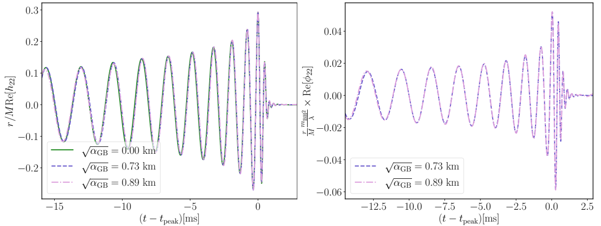
FIG. 8. Gravitational wave radiation (left) and scalar radiation (right) for a BHNS merger where the neutron star is tidally disrupted for different values of the EsGB coupling. We show the real part of the (\ell, m) = (2, 2) spherical harmonic of the strain h and (2, 2) component of \phi both extracted at 100M . Time is measured with respect to the time where |h_{22}| is maximum.
