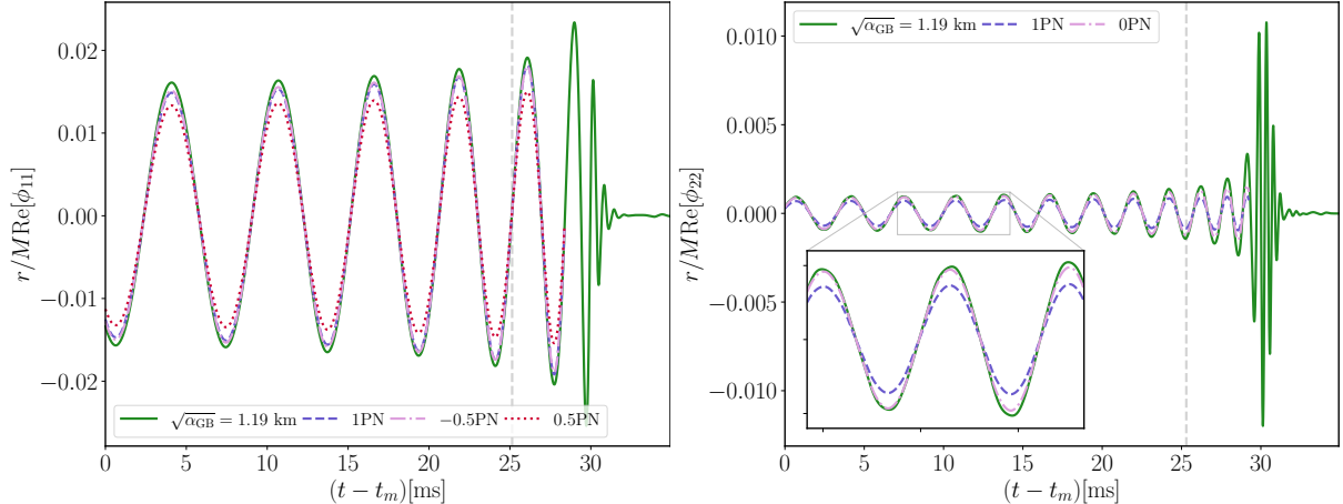
FIG. 4. Scalar radiation for a BHNS binary merger with binary parameters consistent with the GW200115 event for a coupling value of \sqrt{\alpha_{\text{GB}}} = 1.19 km. We show the real part of the (\ell = 2, m = 2) (right) and (\ell = 1, m = 1) (left) spherical harmonic of scalar waveform \phi extracted at 100M . During the inspiral, we also display the PN predictions derived to relative 1.5PN. The vertical line roughly corresponds to time at which modifications to GR are turned off in Ref. [43], i.e. t(f_{\text{insp}} = 0.018/M) . Time is measured with respect to time where both waveforms have a gravitational wave frequency f_m = 0.01/M .
