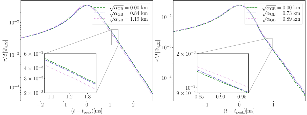
FIG. 6. The amplitude of the \ell = 2, m = 2 spherical harmonic \Psi_4 for a BHNS binary merger with parameters consistent with the GW200115 event (left) and for a binary where the neutron star is tidally disrupted (right) for different values of the EsGB coupling. Time is measured with respect to t_{\text{peak}} , the time where |\Psi_{4,22}| is maximum.
