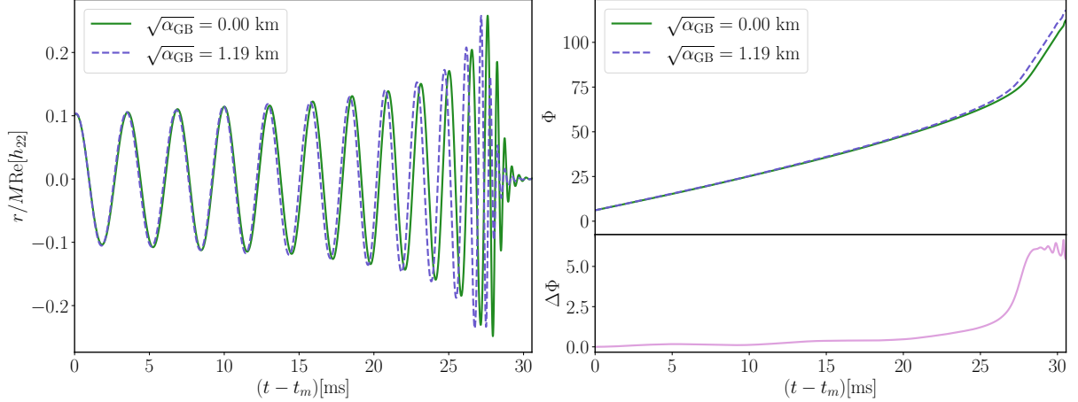
FIG. 2. (Left) Gravitational wave radiation for a BHNS merger with binary parameters consistent with the GW200115 event in GR and EsGB gravity with a coupling value of \sqrt{\alpha_{\text{GB}}} = 1.19 km. We show the real part of the \ell = m = 2 spherical harmonic of the gravitational wave strain h extracted at 100M . (Right) The gravitational wave phase of the aligned waveforms \Phi . The bottom shows the phase difference between the two waveforms \Delta\Phi = \Phi_{\text{GB}} - \Phi_{\text{GR}} . The waveforms have been aligned in time and phase at a gravitational wave frequency f_m = 0.01/M , or equivalently t_m = \{9.7, 8.1\} ms for \sqrt{\alpha_{\text{GB}}} = \{0.0, 1.19\} km according to Eq. 10.
