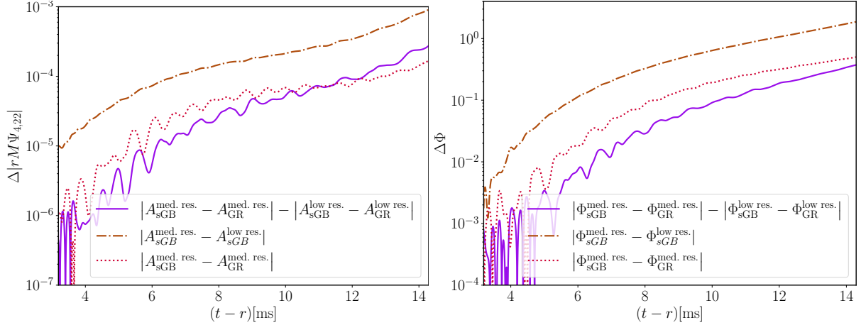
FIG. 11. We show the difference between the low and medium resolutions of the amplitude (left) and phase (right) of the gravitational waveform for the BHNS binary with GW200115 like parameters, an initial separation of D = 8.61M , and coupling of \sqrt{\alpha_{\text{GB}}} = 1.19\text{km} . We also show the difference between the EsGB and GR amplitude and phase at low and medium resolutions (dashed brown line). This provides evidence that the truncation error roughly cancels between the EsGB and GR runs.
