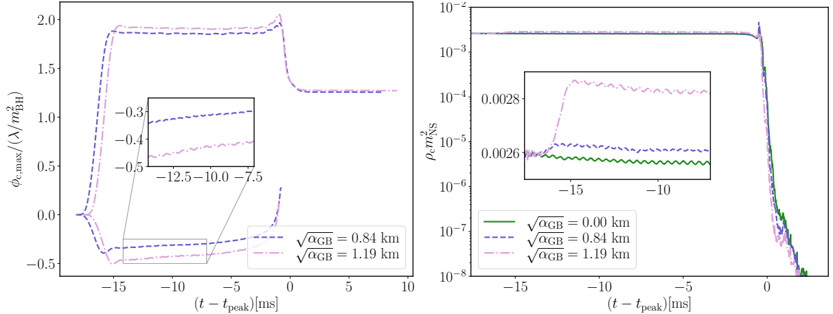
FIG. 12. Left: The maximum value of the scalar field over the numerical domain (excluding black hole interior) and value of the scalar field at the center of the neutron star (which is negative for most of the evolution). Right: The maximum rest-mass density (located at center neutron star). These results are for the GW200115-like BHNS merger and various EsGB coupling values.
