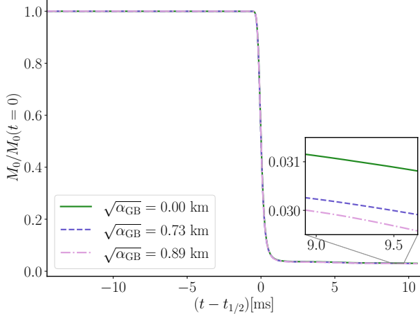
FIG. 9. The total fluid rest mass outside black hole horizon for the merger where the neutron star is tidally disrupted for different values of the EsGB coupling. Time is measured with respect to the time where half of the neutron star mass has been accreted onto black hole t_{1/2} and the rest mass is normalized by its initial value.
