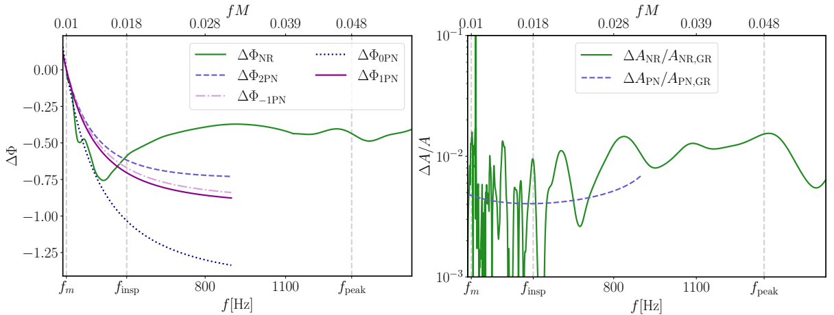
FIG. 3. PN and numerical predictions for the dephasing (left) and correction to the amplitude (right) of gravitational waveform of the binary shown in Fig. 2 (see Eq.11, 12, 12 and 13). We also show the dephasing when only considering leading order (dipolar) contribution to phase and all contributions up to 0PN and 1PN order. The first vertical line corresponds to frequency at which waveforms are aligned f_m according to Eq.10, the second line to the end of inspiral stage in GR f_{\text{insp}} , and the third to frequency at which amplitude of GR waveform peaks f_{\text{peak}} .
