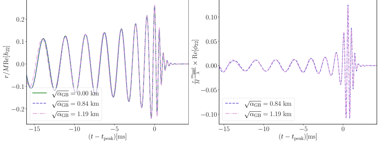
FIG. 5. Gravitational wave radiation (left) and scalar radiation (right) for a BHNS merger with binary parameters consistent with the GW200115 event for different values of the EsGB coupling. We show the real part of the ( \ell = 2, m = 2 ) spherical harmonic of the strain h and (2, 2) component of \phi both extracted at 100M . Time is measured with respect to the time where amplitude of h_{22} is maximum t_{\text{peak}} .
